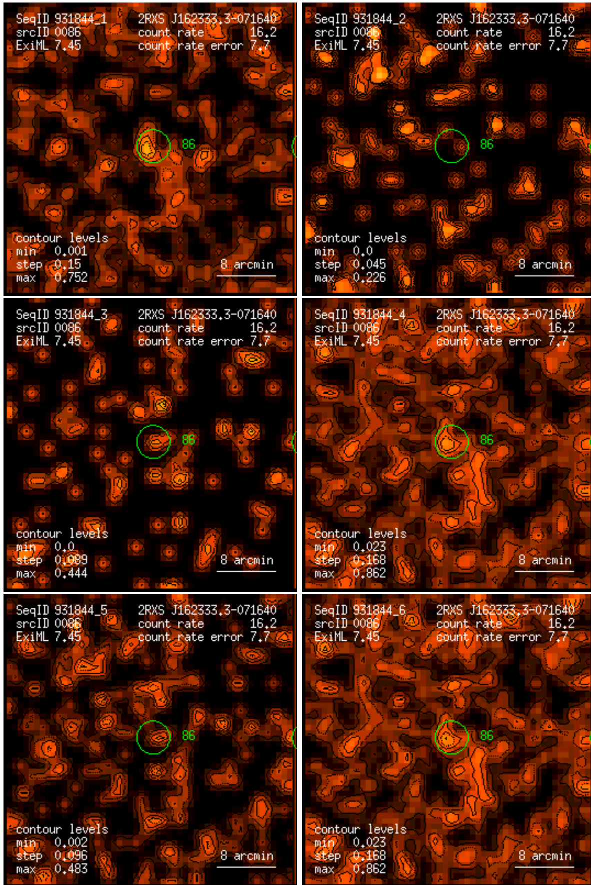
Figure 86: RASS 931844: detection 0086: band rate images, Gaussian filter: (1) PSPC channels 11 – 41, (2) 52 – 90, (3) 91 – 201, (4) 11 – 235, (5) 52 – 201, (6) 11 – 201. Broad band rates in counts/ks. Band rate contour levels in counts/ks/arcmin 2 .
