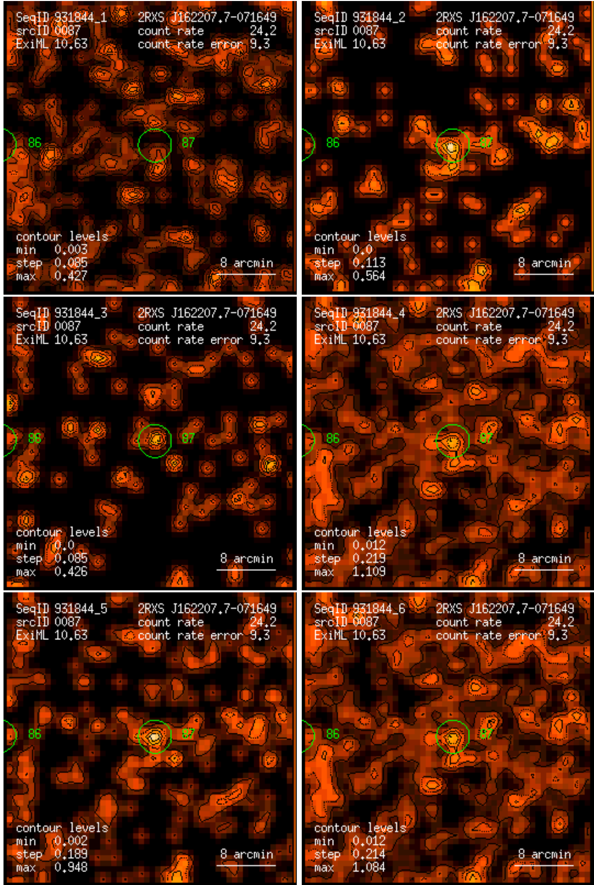
Figure 87: RASS 931844: detection 0087: band rate images, Gaussian filter: (1) PSPC channels 11 – 41, (2) 52 – 90, (3) 91 – 201, (4) 11 – 235, (5) 52 – 201, (6) 11 – 201. Broad band rates in counts/ks. Band rate contour levels in counts/ks/arcmin 2 .
