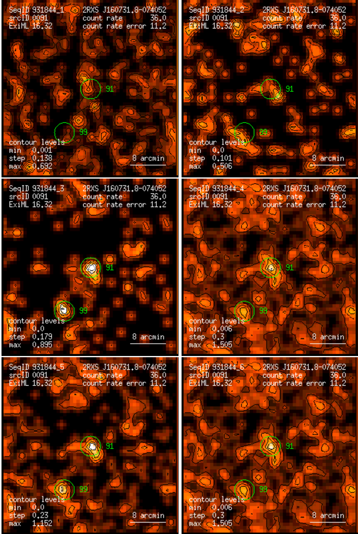
Figure 91: RASS 931844: detection 0091: band rate images, Gaussian filter: (1) PSPC channels 11 – 41, (2) 52 – 90, (3) 91 – 201, (4) 11 – 235, (5) 52 – 201, (6) 11 – 201. Broad band rates in counts/ks. Band rate contour levels in counts/ks/arcmin 2 .
