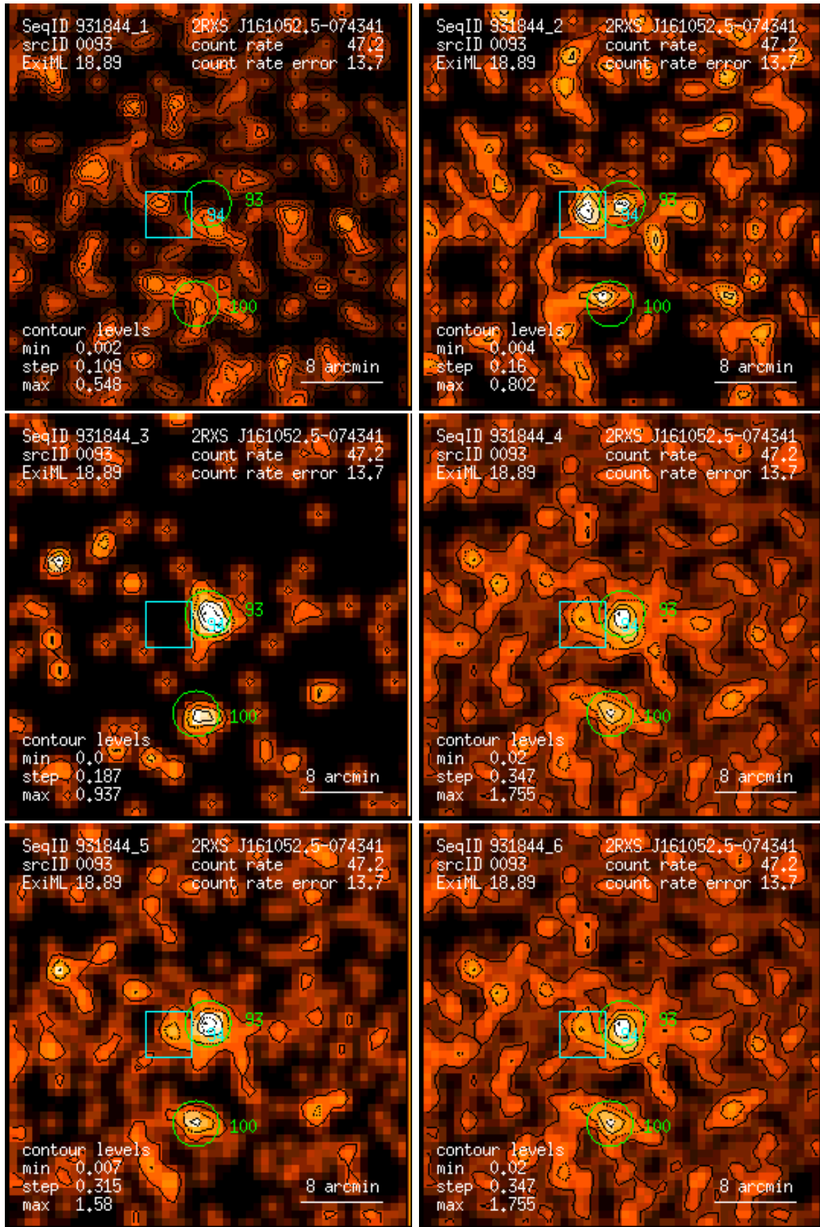
Figure 93: RASS 931844: detection 0093: band rate images, Gaussian filter: (1) PSPC channels 11 – 41, (2) 52 – 90, (3) 91 – 201, (4) 11 – 235, (5) 52 – 201, (6) 11 – 201. Broad band rates in counts/ks. Band rate contour levels in counts/ks/arcmin 2 .
