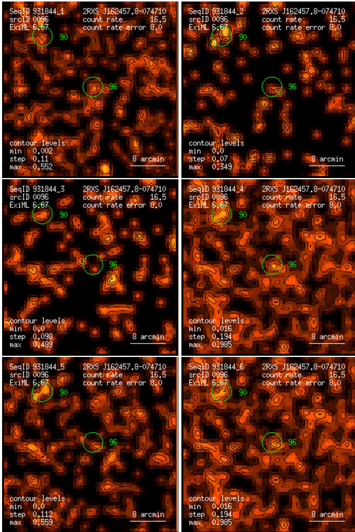
Figure 96: RASS 931844: detection 0096: band rate images, Gaussian filter: (1) PSPC channels 11 – 41, (2) 52 – 90, (3) 91 – 201, (4) 11 – 235, (5) 52 – 201, (6) 11 – 201. Broad band rates in counts/ks. Band rate contour levels in counts/ks/arcmin 2 .
