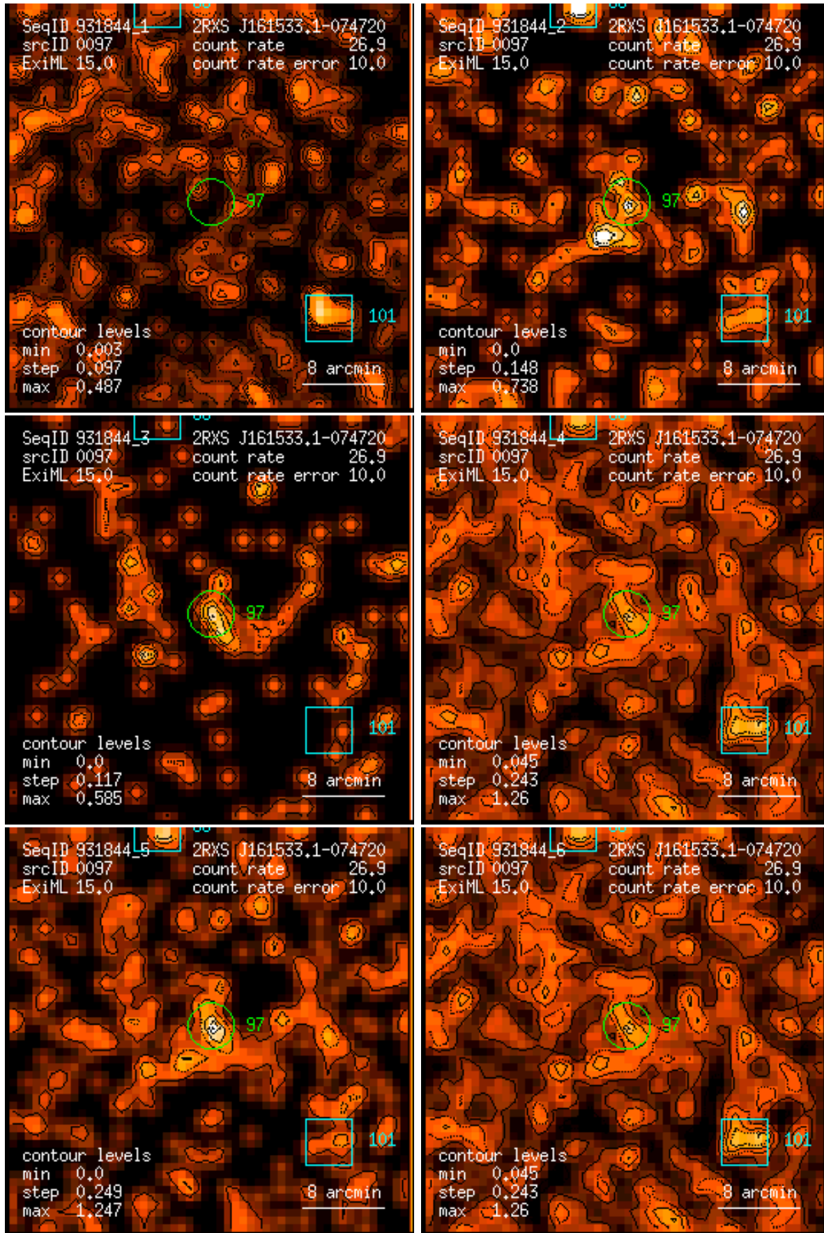
Figure 97: RASS 931844: detection 0097: band rate images, Gaussian filter: (1) PSPC channels 11 – 41, (2) 52 – 90, (3) 91 – 201, (4) 11 – 235, (5) 52 – 201, (6) 11 – 201. Broad band rates in counts/ks. Band rate contour levels in counts/ks/arcmin 2 .
