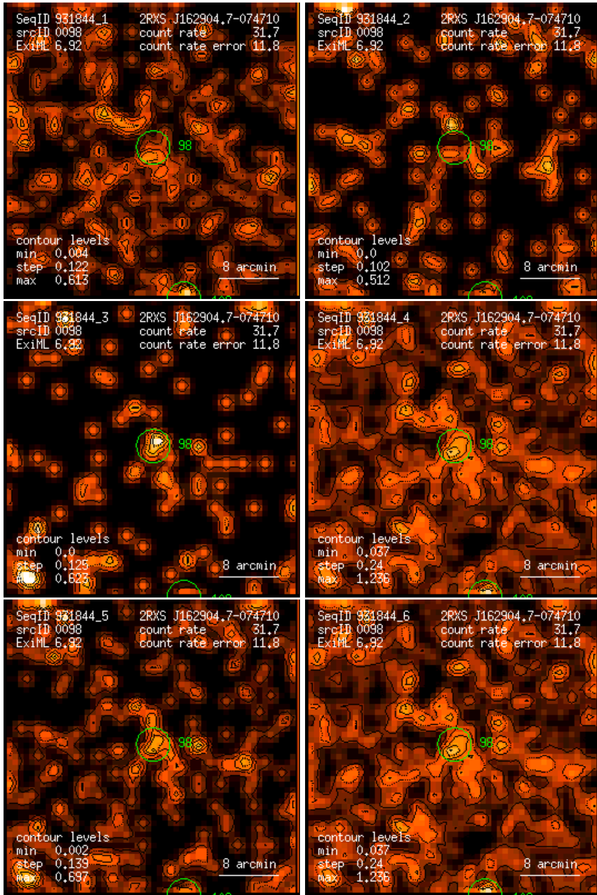
Figure 98: RASS 931844: detection 0098: band rate images, Gaussian filter: (1) PSPC channels 11 – 41, (2) 52 – 90, (3) 91 – 201, (4) 11 – 235, (5) 52 – 201, (6) 11 – 201. Broad band rates in counts/ks. Band rate contour levels in counts/ks/arcmin 2 .
