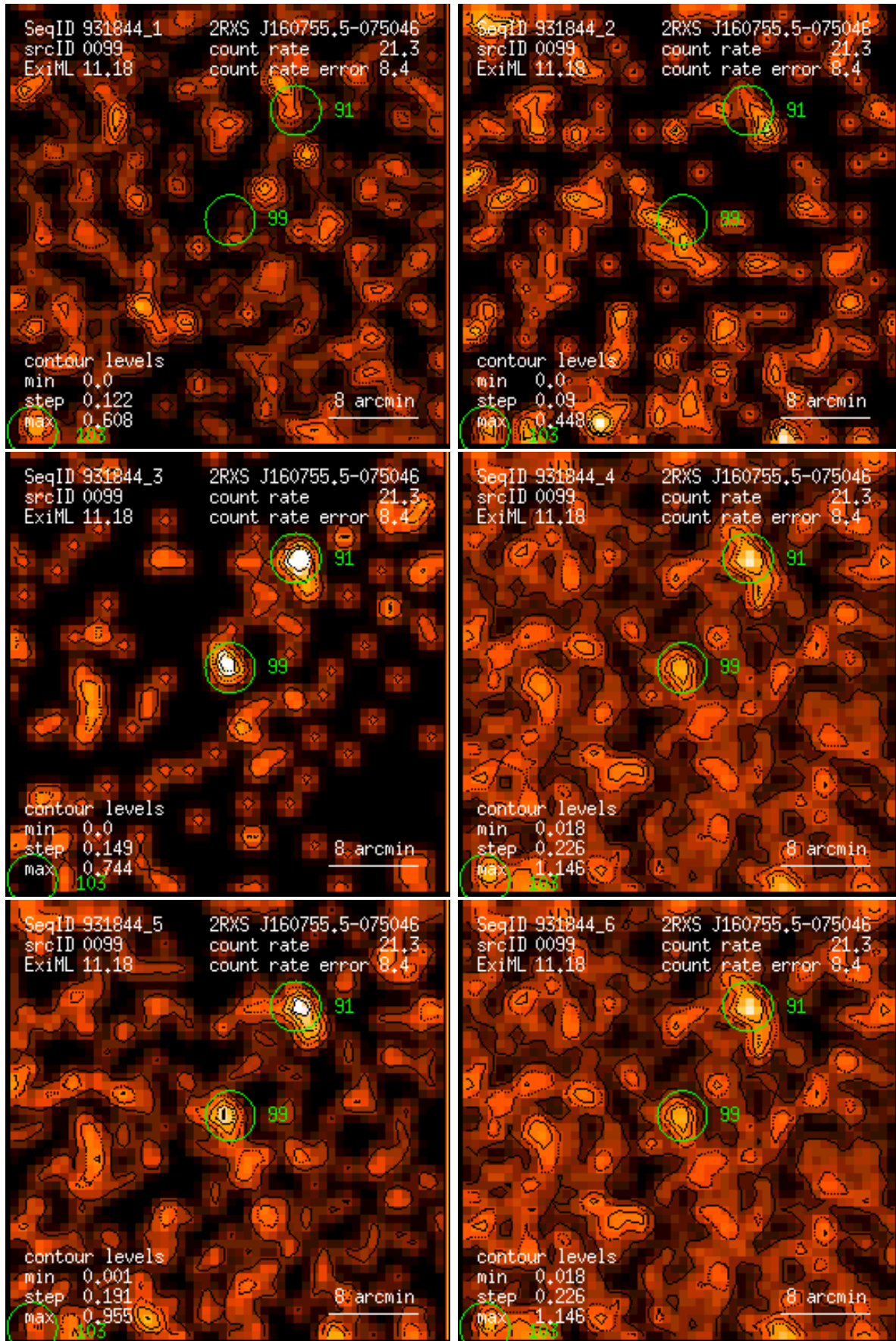
Figure 99: RASS 931844: detection 0099: band rate images, Gaussian filter: (1) PSPC channels 11 – 41, (2) 52 – 90, (3) 91 – 201, (4) 11 – 235, (5) 52 – 201, (6) 11 – 201. Broad band rates in counts/ks. Band rate contour levels in counts/ks/arcmin 2 .
