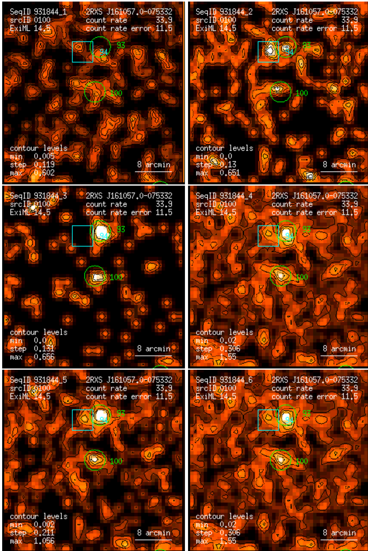
Figure 100: RASS 931844: detection 0100: band rate images, Gaussian filter: (1) PSPC channels 11 – 41, (2) 52 – 90, (3) 91 – 201, (4) 11 – 235, (5) 52 – 201, (6) 11 – 201. Broad band rates in counts/ks. Band rate contour levels in counts/ks/arcmin 2 .
