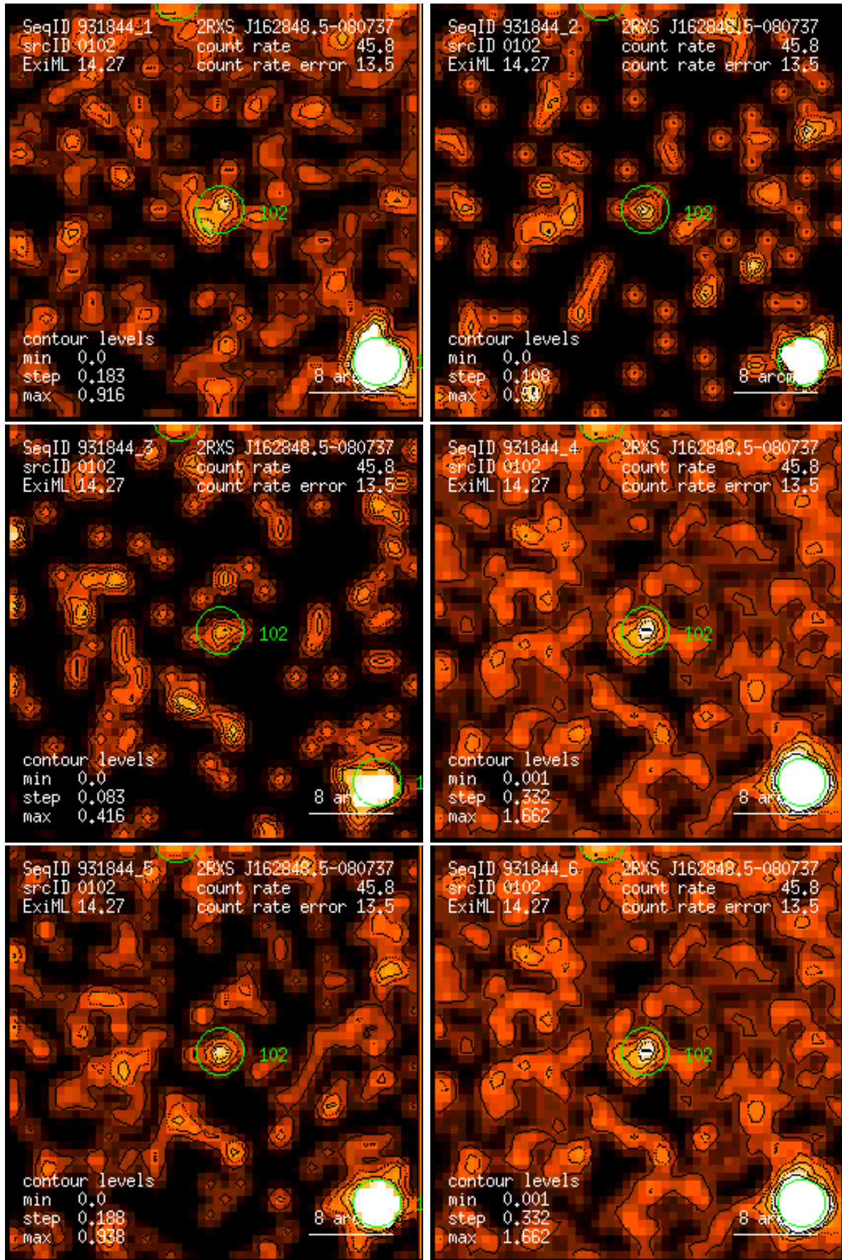
Figure 102: RASS 931844: detection 0102: band rate images, Gaussian filter: (1) PSPC channels 11 – 41, (2) 52 – 90, (3) 91 – 201, (4) 11 – 235, (5) 52 – 201, (6) 11 – 201. Broad band rates in counts/ks. Band rate contour levels in counts/ks/arcmin 2 .
