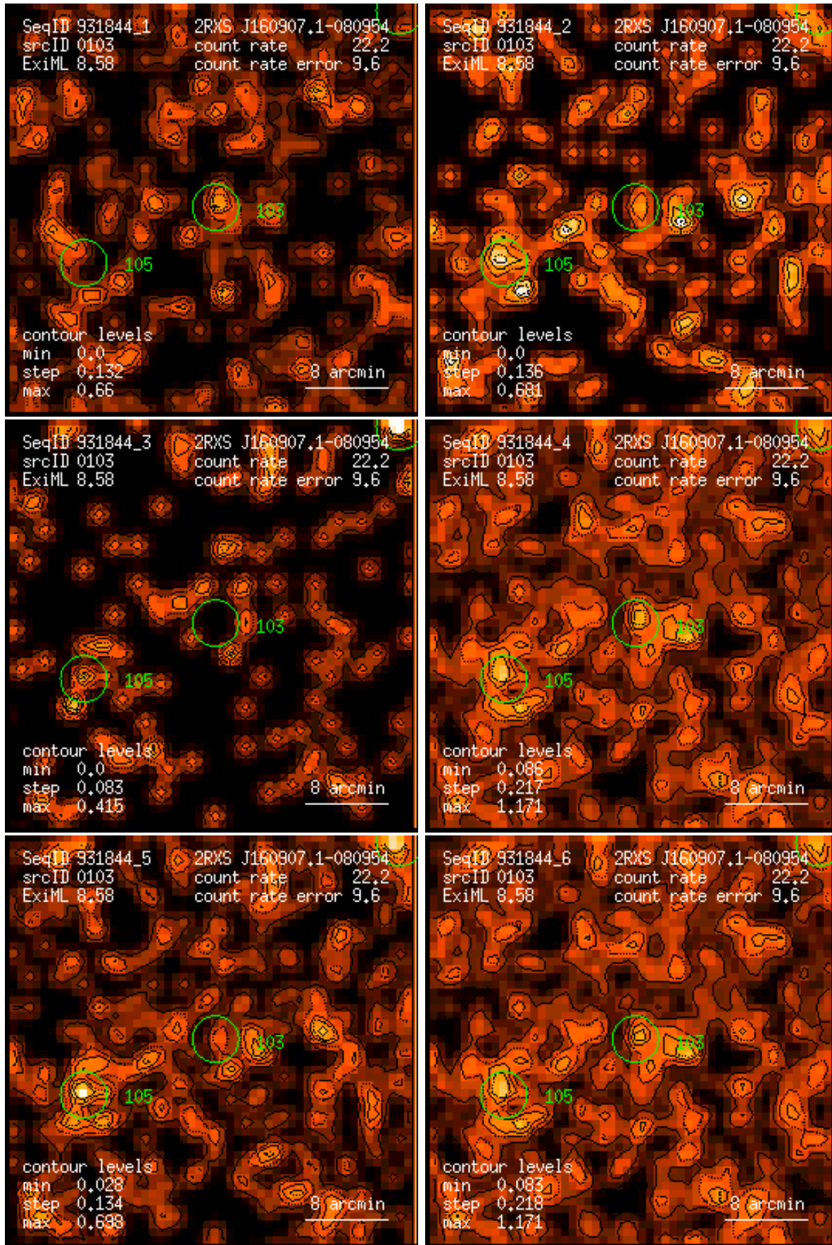
Figure 103: RASS 931844: detection 0103: band rate images, Gaussian filter: (1) PSPC channels 11 – 41, (2) 52 – 90, (3) 91 – 201, (4) 11 – 235, (5) 52 – 201, (6) 11 – 201. Broad band rates in counts/ks. Band rate contour levels in counts/ks/arcmin 2 .
