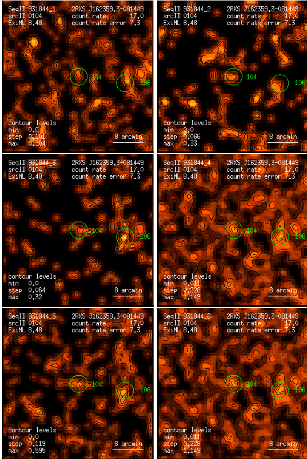
Figure 104: RASS 931844: detection 0104: band rate images, Gaussian filter: (1) PSPC channels 11 – 41, (2) 52 – 90, (3) 91 – 201, (4) 11 – 235, (5) 52 – 201, (6) 11 – 201. Broad band rates in counts/ks. Band rate contour levels in counts/ks/arcmin 2 .
