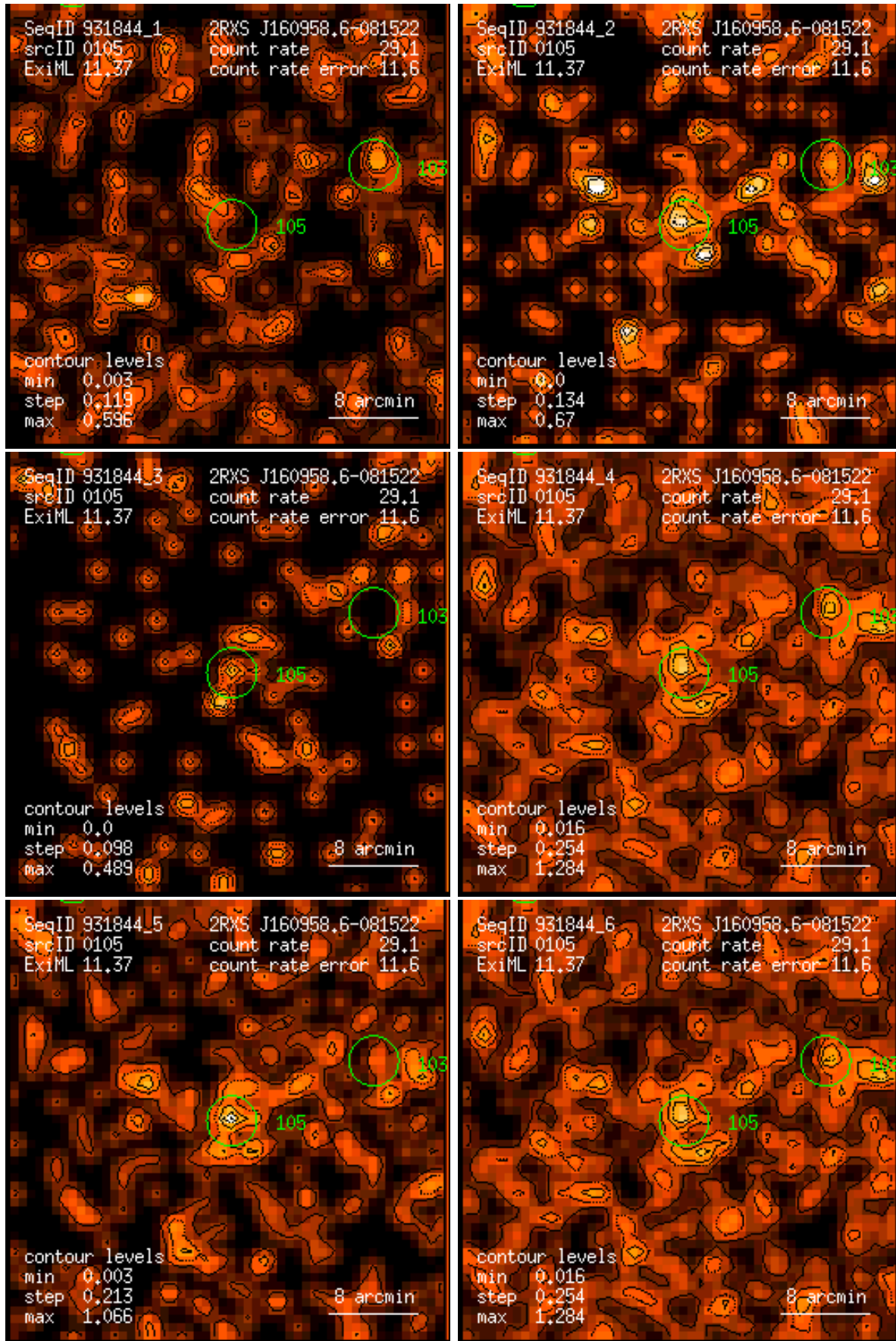
Figure 105: RASS 931844: detection 0105: band rate images, Gaussian filter: (1) PSPC channels 11 – 41, (2) 52 – 90, (3) 91 – 201, (4) 11 – 235, (5) 52 – 201, (6) 11 – 201. Broad band rates in counts/ks. Band rate contour levels in counts/ks/arcmin 2 .
