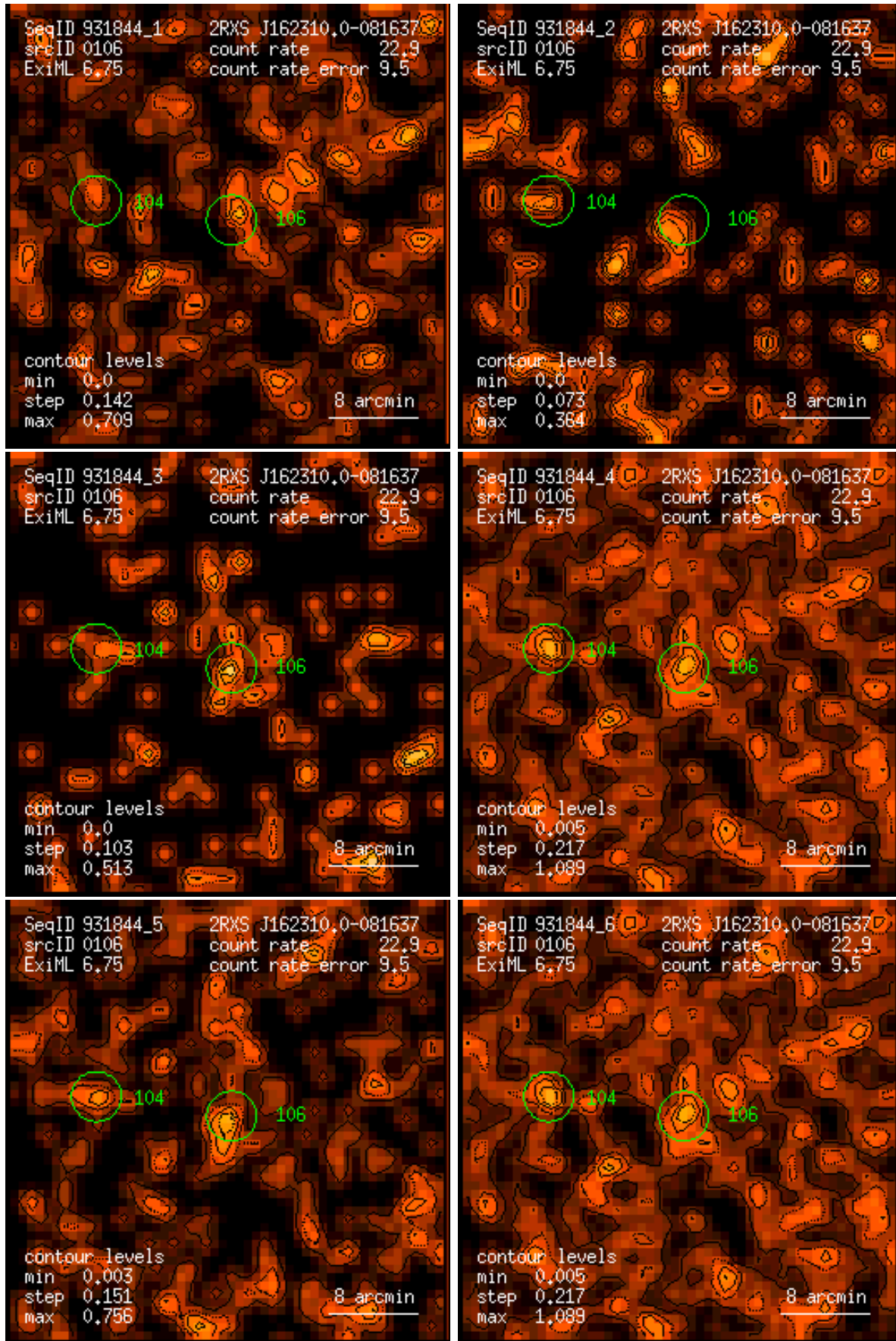
Figure 106: RASS 931844: detection 0106: band rate images, Gaussian filter: (1) PSPC channels 11 – 41, (2) 52 – 90, (3) 91 – 201, (4) 11 – 235, (5) 52 – 201, (6) 11 – 201. Broad band rates in counts/ks. Band rate contour levels in counts/ks/arcmin 2 .
