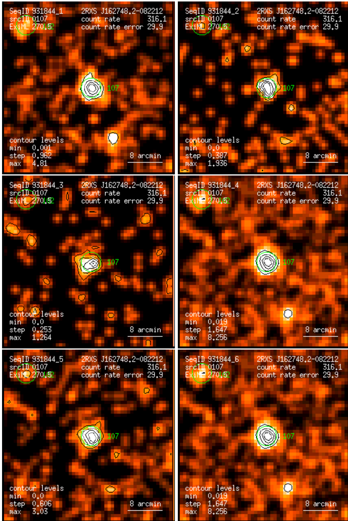
Figure 107: RASS 931844: detection 0107: band rate images, Gaussian filter: (1) PSPC channels 11 – 41, (2) 52 – 90, (3) 91 – 201, (4) 11 – 235, (5) 52 – 201, (6) 11 – 201. Broad band rates in counts/ks. Band rate contour levels in counts/ks/arcmin 2 .
