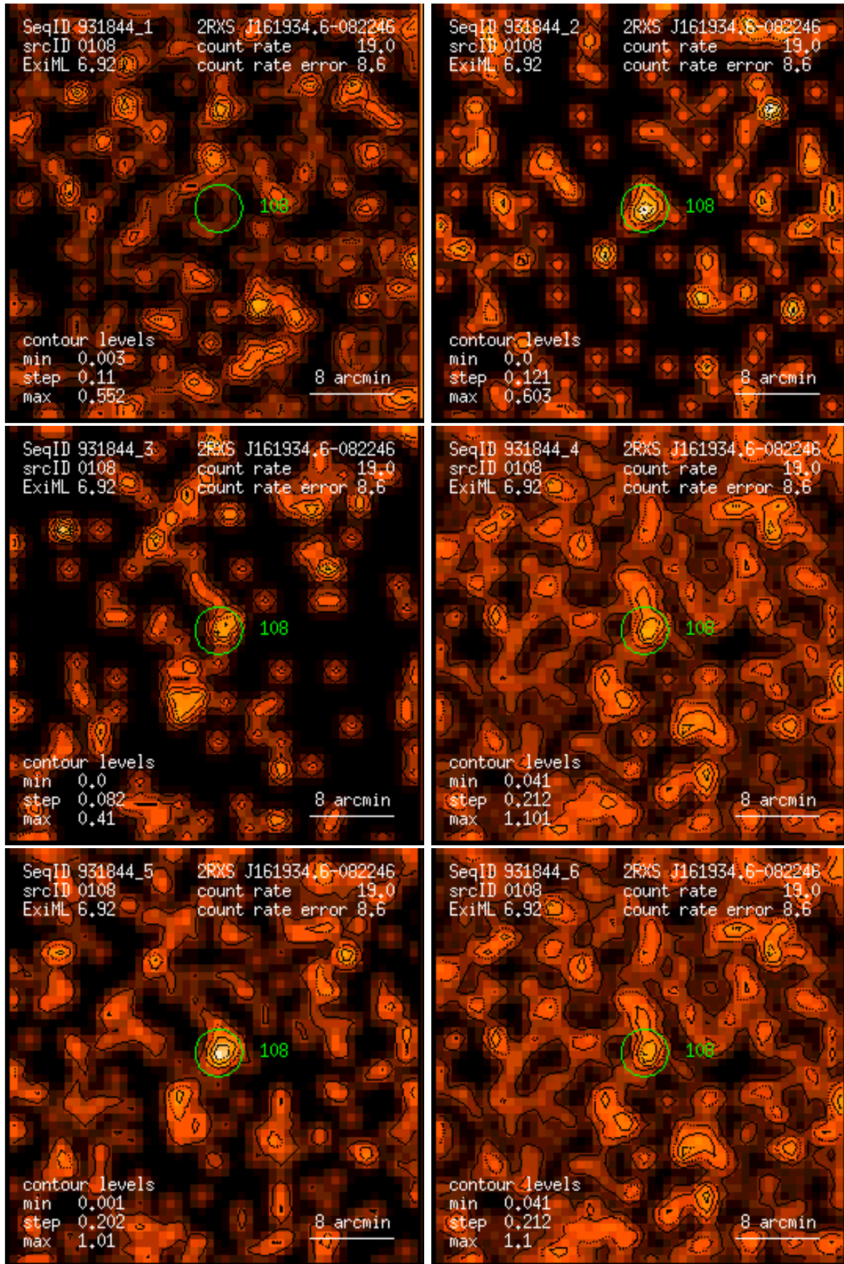
Figure 108: RASS 931844: detection 0108: band rate images, Gaussian filter: (1) PSPC channels 11 – 41, (2) 52 – 90, (3) 91 – 201, (4) 11 – 235, (5) 52 – 201, (6) 11 – 201. Broad band rates in counts/ks. Band rate contour levels in counts/ks/arcmin 2 .
