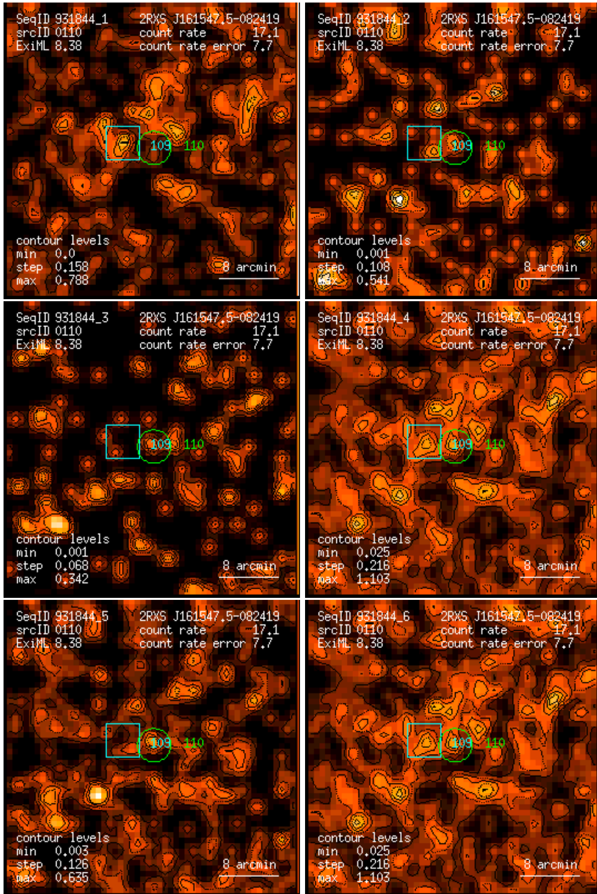
Figure 110: RASS 931844: detection 0110: band rate images, Gaussian filter: (1) PSPC channels 11 – 41, (2) 52 – 90, (3) 91 – 201, (4) 11 – 235, (5) 52 – 201, (6) 11 – 201. Broad band rates in counts/ks. Band rate contour levels in counts/ks/arcmin 2 .
