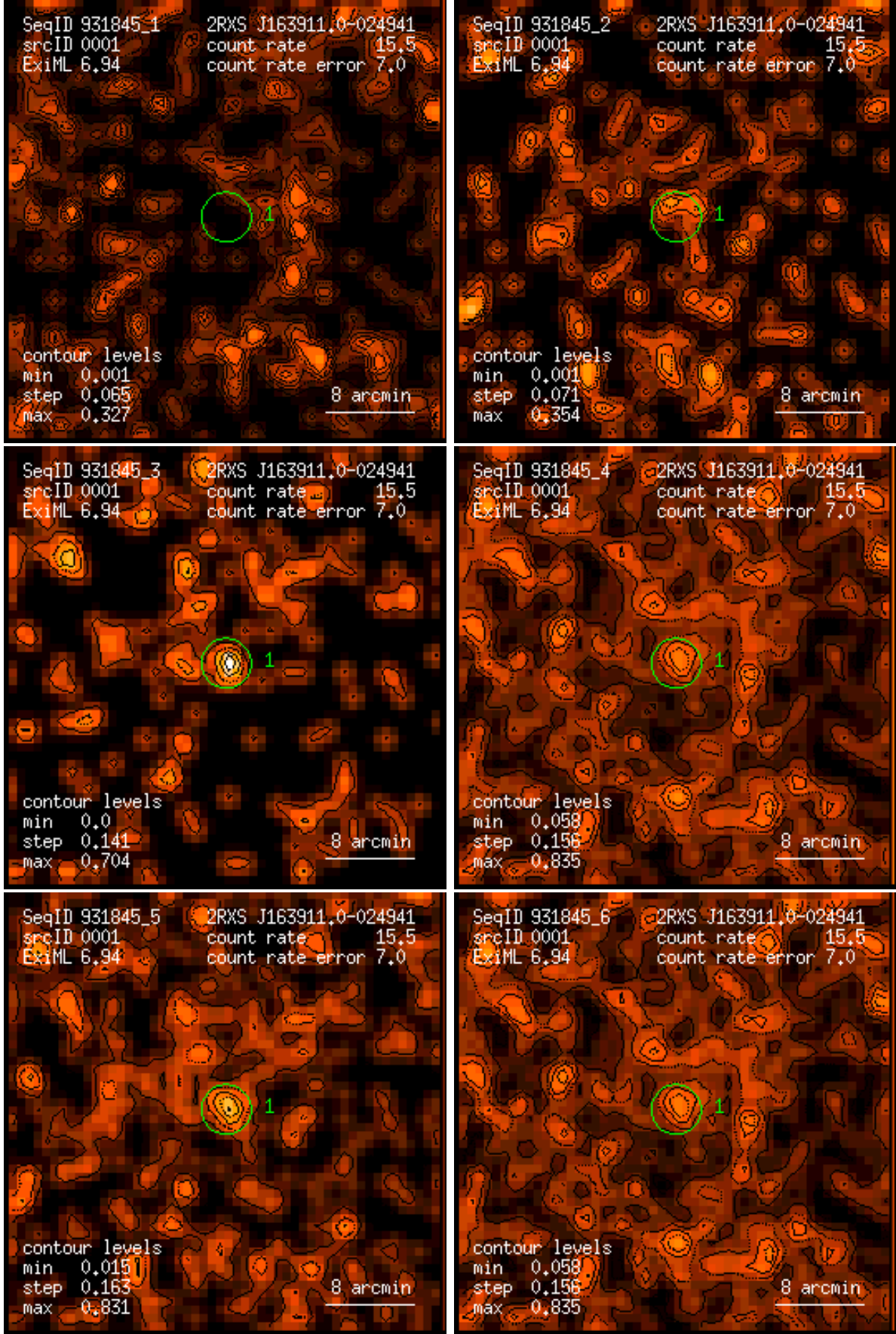
Figure 1: RASS 931845: detection 0001: band rate images, Gaussian filter: (1) PSPC channels 11 – 41, (2) 52 – 90, (3) 91 – 201, (4) 11 – 235, (5) 52 – 201, (6) 11 – 201. Broad band rates in counts/ks. Band rate contour levels in counts/ks/arcmin 2 .
