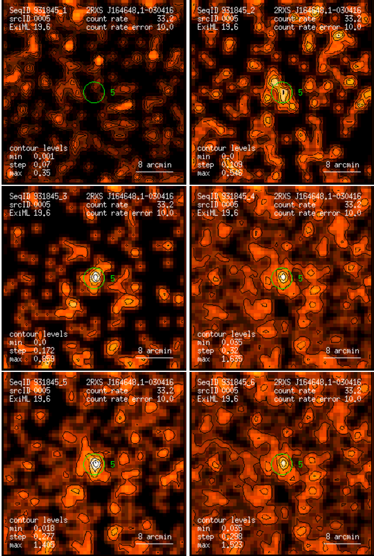
Figure 5: RASS 931845: detection 0005: band rate images, Gaussian filter: (1) PSPC channels 11 – 41, (2) 52 – 90, (3) 91 – 201, (4) 11 – 235, (5) 52 – 201, (6) 11 – 201. Broad band rates in counts/ks. Band rate contour levels in counts/ks/arcmin 2 .
