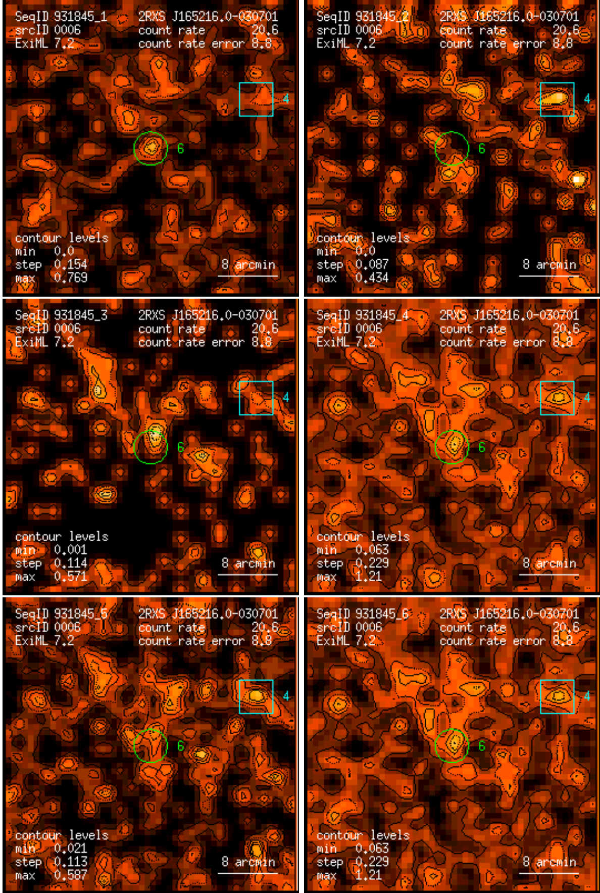
Figure 6: RASS 931845: detection 0006: band rate images, Gaussian filter: (1) PSPC channels 11 – 41, (2) 52 – 90, (3) 91 – 201, (4) 11 – 235, (5) 52 – 201, (6) 11 – 201. Broad band rates in counts/ks. Band rate contour levels in counts/ks/arcmin 2 .
