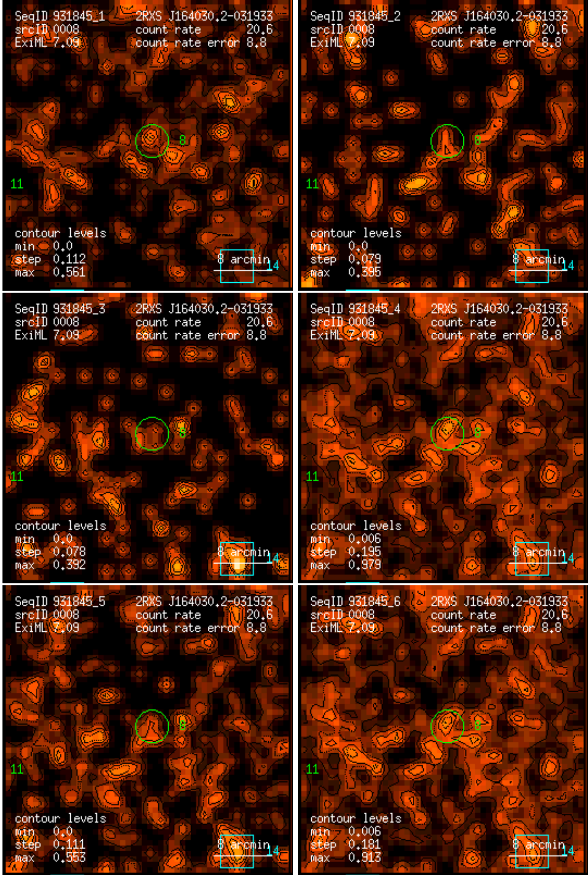
Figure 8: RASS 931845: detection 0008: band rate images, Gaussian filter: (1) PSPC channels 11 – 41, (2) 52 – 90, (3) 91 – 201, (4) 11 – 235, (5) 52 – 201, (6) 11 – 201. Broad band rates in counts/ks. Band rate contour levels in counts/ks/arcmin 2 .
