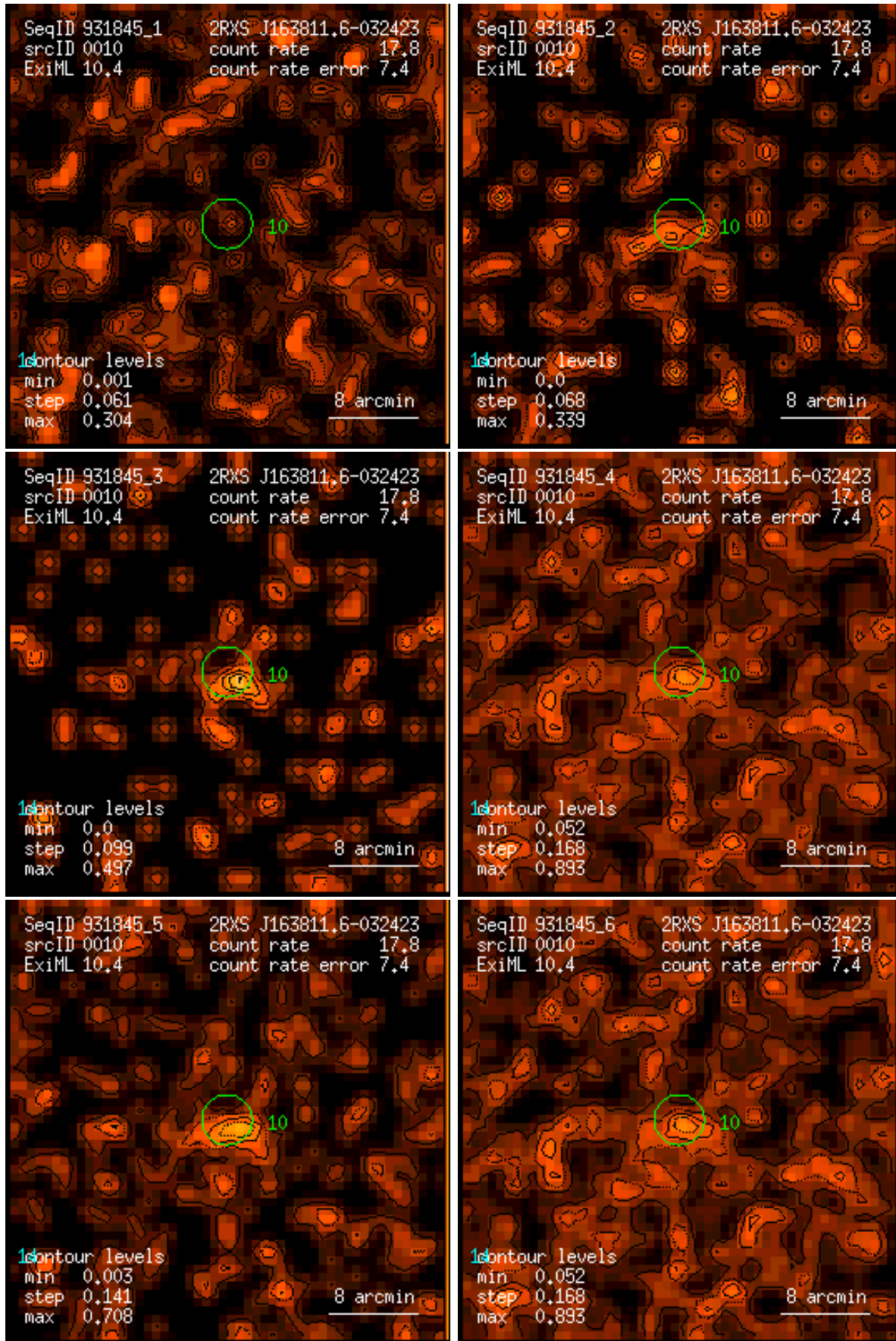
Figure 10: RASS 931845: detection 0010: band rate images, Gaussian filter: (1) PSPC channels 11 – 41, (2) 52 – 90, (3) 91 – 201, (4) 11 – 235, (5) 52 – 201, (6) 11 – 201. Broad band rates in counts/ks. Band rate contour levels in counts/ks/arcmin 2 .
