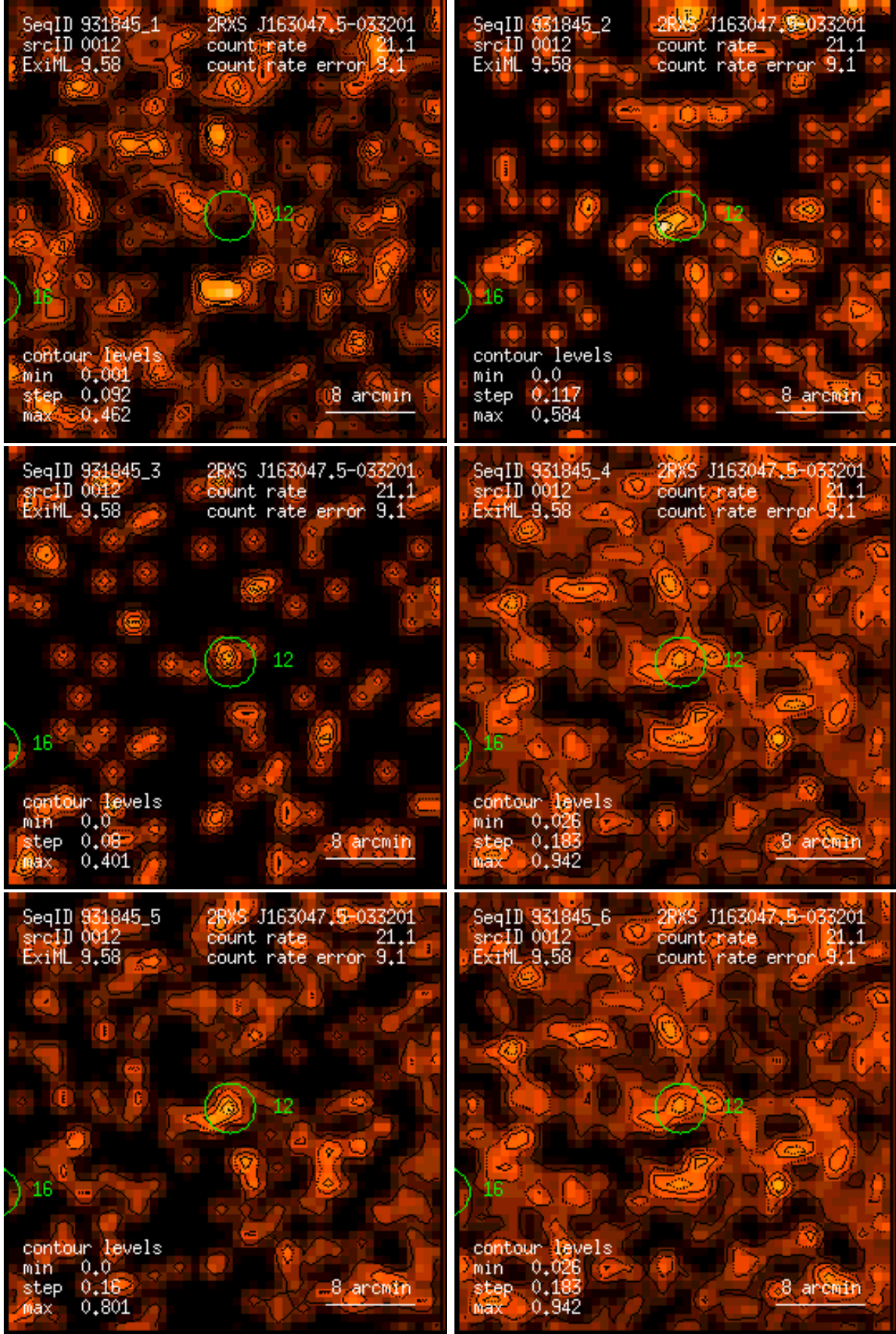
Figure 12: RASS 931845: detection 0012: band rate images, Gaussian filter: (1) PSPC channels 11 – 41, (2) 52 – 90, (3) 91 – 201, (4) 11 – 235, (5) 52 – 201, (6) 11 – 201. Broad band rates in counts/ks. Band rate contour levels in counts/ks/arcmin 2 .
