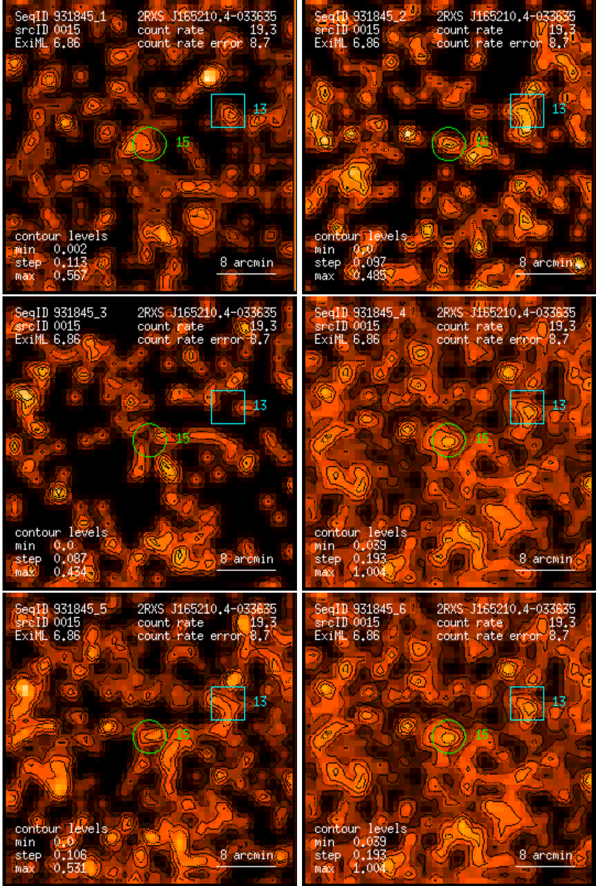
Figure 15: RASS 931845: detection 0015: band rate images, Gaussian filter: (1) PSPC channels 11 – 41, (2) 52 – 90, (3) 91 – 201, (4) 11 – 235, (5) 52 – 201, (6) 11 – 201. Broad band rates in counts/ks. Band rate contour levels in counts/ks/arcmin 2 .
