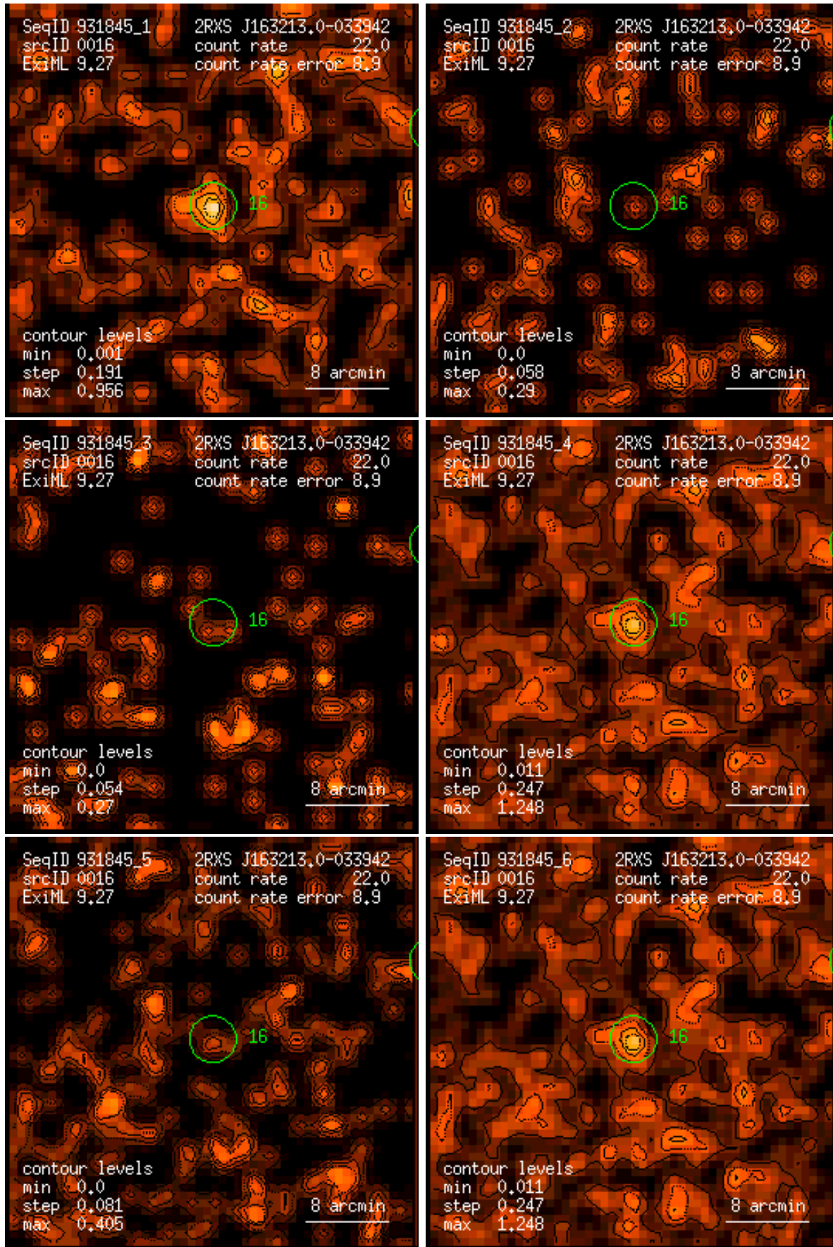
Figure 16: RASS 931845: detection 0016: band rate images, Gaussian filter: (1) PSPC channels 11 – 41, (2) 52 – 90, (3) 91 – 201, (4) 11 – 235, (5) 52 – 201, (6) 11 – 201. Broad band rates in counts/ks. Band rate contour levels in counts/ks/arcmin 2 .
