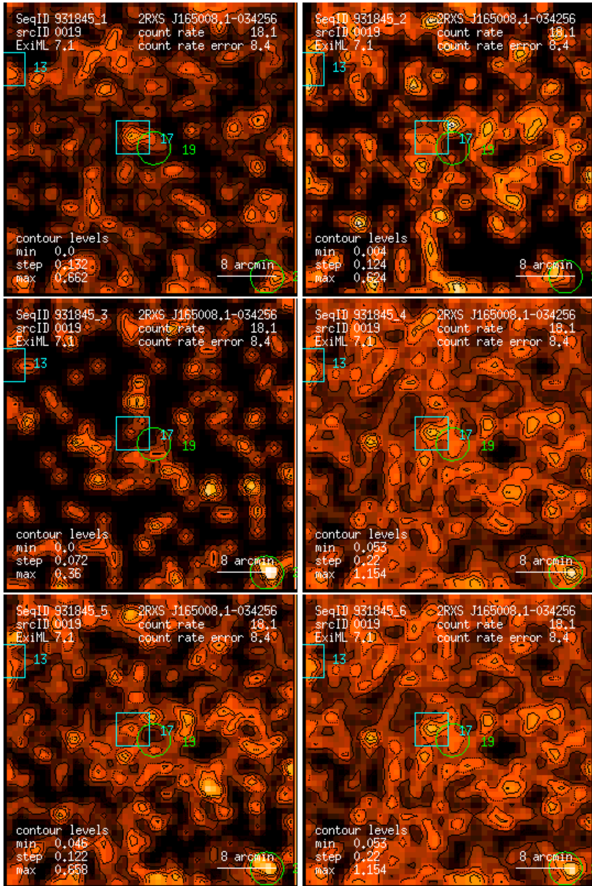
Figure 19: RASS 931845: detection 0019: band rate images, Gaussian filter: (1) PSPC channels 11 – 41, (2) 52 – 90, (3) 91 – 201, (4) 11 – 235, (5) 52 – 201, (6) 11 – 201. Broad band rates in counts/ks. Band rate contour levels in counts/ks/arcmin 2 .
