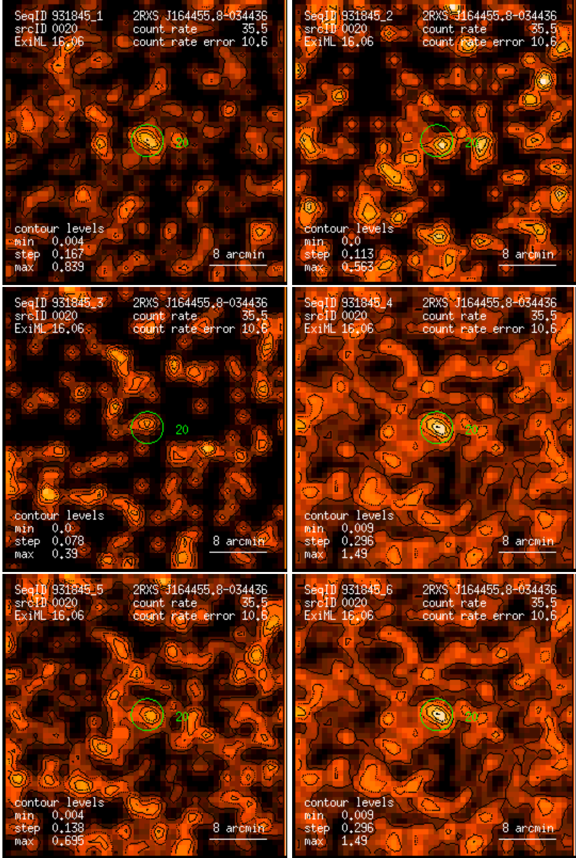
Figure 20: RASS 931845: detection 0020: band rate images, Gaussian filter: (1) PSPC channels 11 – 41, (2) 52 – 90, (3) 91 – 201, (4) 11 – 235, (5) 52 – 201, (6) 11 – 201. Broad band rates in counts/ks. Band rate contour levels in counts/ks/arcmin 2 .
