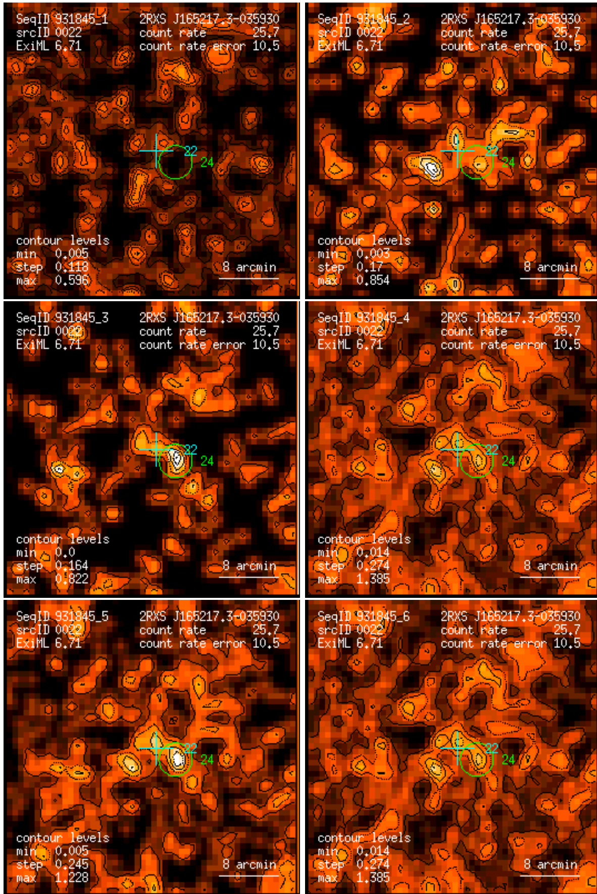
Figure 22: RASS 931845: detection 0022: band rate images, Gaussian filter: (1) PSPC channels 11 – 41, (2) 52 – 90, (3) 91 – 201, (4) 11 – 235, (5) 52 – 201, (6) 11 – 201. Broad band rates in counts/ks. Band rate contour levels in counts/ks/arcmin 2 .
