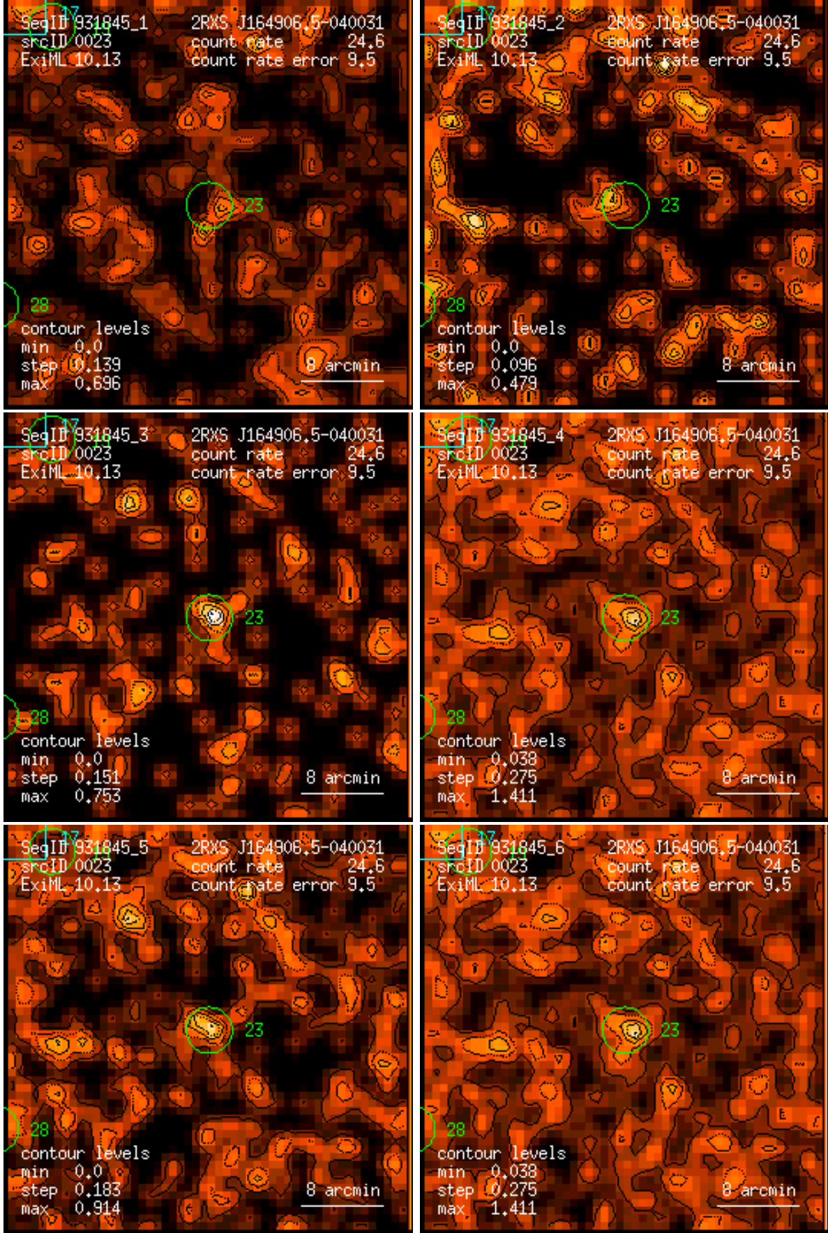
Figure 23: RASS 931845: detection 0023: band rate images, Gaussian filter: (1) PSPC channels 11 – 41, (2) 52 – 90, (3) 91 – 201, (4) 11 – 235, (5) 52 – 201, (6) 11 – 201. Broad band rates in counts/ks. Band rate contour levels in counts/ks/arcmin 2 .
