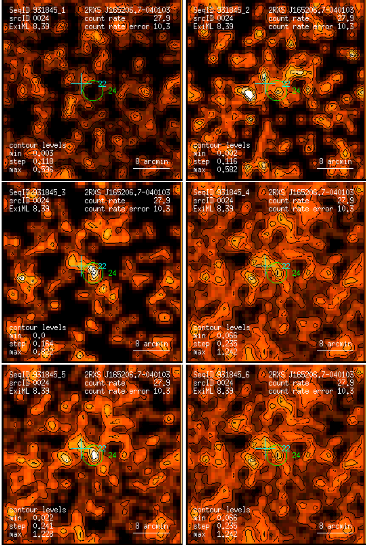
Figure 24: RASS 931845: detection 0024: band rate images, Gaussian filter: (1) PSPC channels 11 – 41, (2) 52 – 90, (3) 91 – 201, (4) 11 – 235, (5) 52 – 201, (6) 11 – 201. Broad band rates in counts/ks. Band rate contour levels in counts/ks/arcmin 2 .
