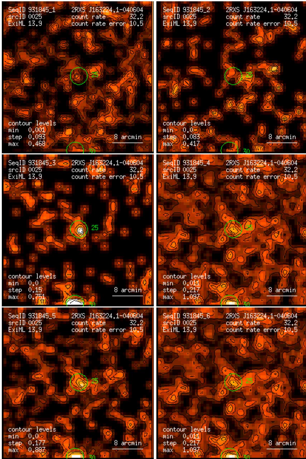
Figure 25: RASS 931845: detection 0025: band rate images, Gaussian filter: (1) PSPC channels 11 – 41, (2) 52 – 90, (3) 91 – 201, (4) 11 – 235, (5) 52 – 201, (6) 11 – 201. Broad band rates in counts/ks. Band rate contour levels in counts/ks/arcmin 2 .
