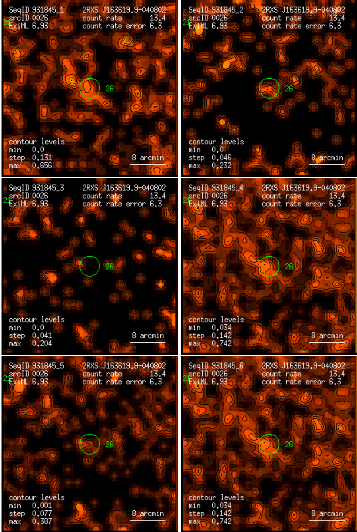
Figure 26: RASS 931845: detection 0026: band rate images, Gaussian filter: (1) PSPC channels 11 – 41, (2) 52 – 90, (3) 91 – 201, (4) 11 – 235, (5) 52 – 201, (6) 11 – 201. Broad band rates in counts/ks. Band rate contour levels in counts/ks/arcmin 2 .
