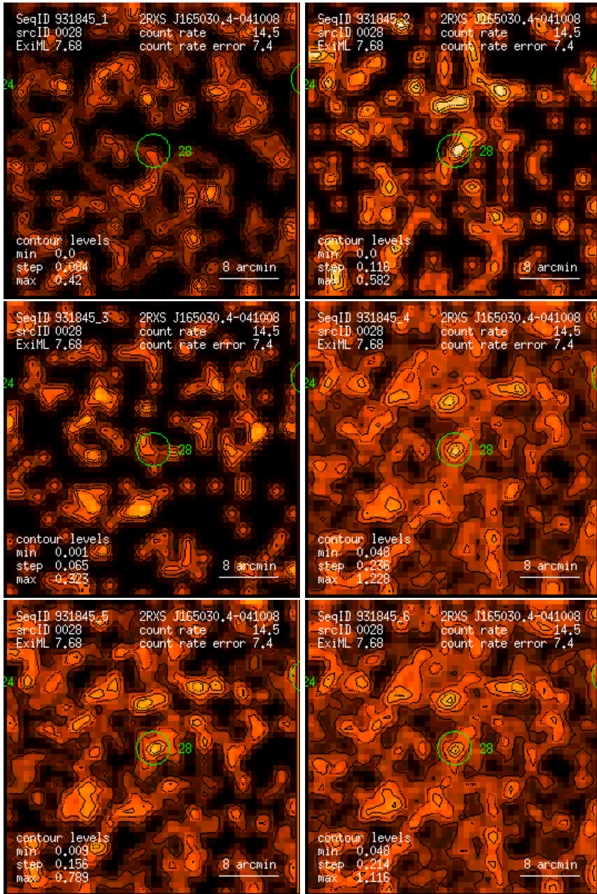
Figure 28: RASS 931845: detection 0028: band rate images, Gaussian filter: (1) PSPC channels 11 – 41, (2) 52 – 90, (3) 91 – 201, (4) 11 – 235, (5) 52 – 201, (6) 11 – 201. Broad band rates in counts/ks. Band rate contour levels in counts/ks/arcmin 2 .
