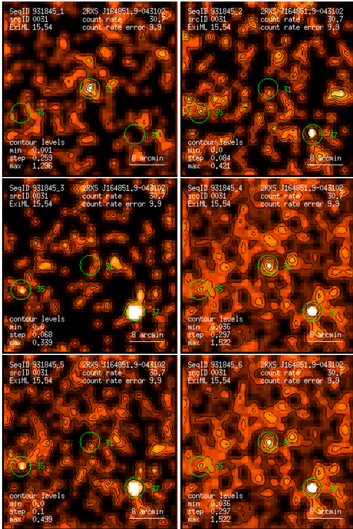
Figure 31: RASS 931845: detection 0031: band rate images, Gaussian filter: (1) PSPC channels 11 – 41, (2) 52 – 90, (3) 91 – 201, (4) 11 – 235, (5) 52 – 201, (6) 11 – 201. Broad band rates in counts/ks. Band rate contour levels in counts/ks/arcmin 2 .
