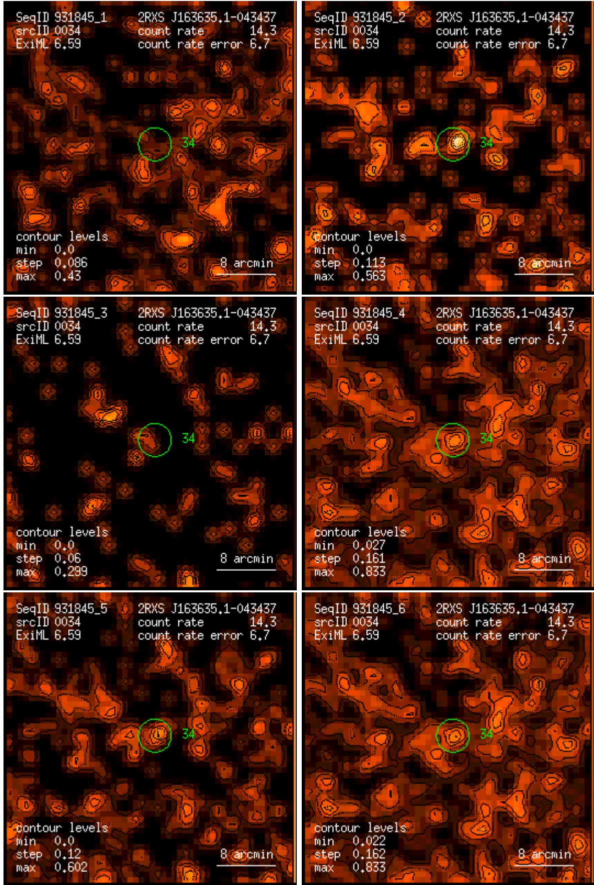
Figure 34: RASS 931845: detection 0034: band rate images, Gaussian filter: (1) PSPC channels 11 – 41, (2) 52 – 90, (3) 91 – 201, (4) 11 – 235, (5) 52 – 201, (6) 11 – 201. Broad band rates in counts/ks. Band rate contour levels in counts/ks/arcmin 2 .
