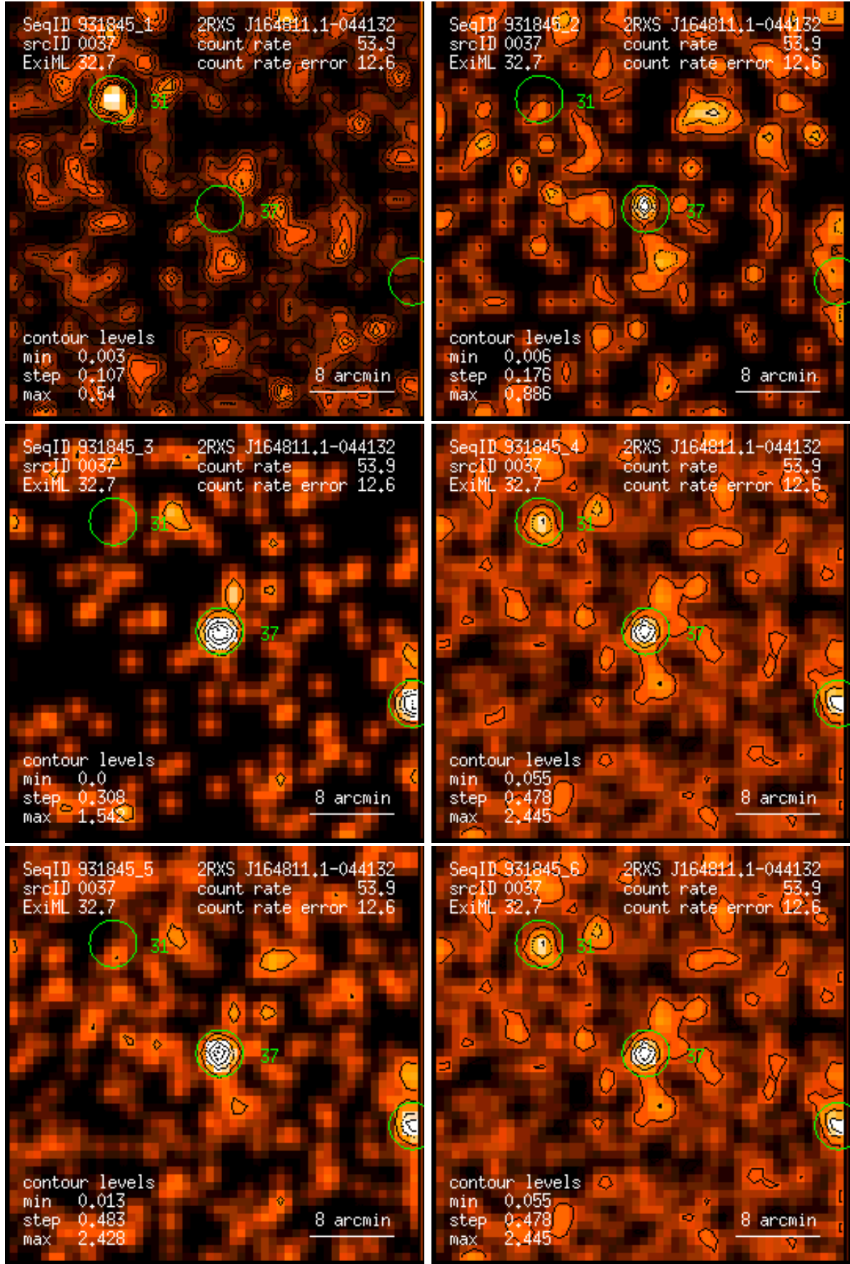
Figure 37: RASS 931845: detection 0037: band rate images, Gaussian filter: (1) PSPC channels 11 – 41, (2) 52 – 90, (3) 91 – 201, (4) 11 – 235, (5) 52 – 201, (6) 11 – 201. Broad band rates in counts/ks. Band rate contour levels in counts/ks/arcmin 2 .
