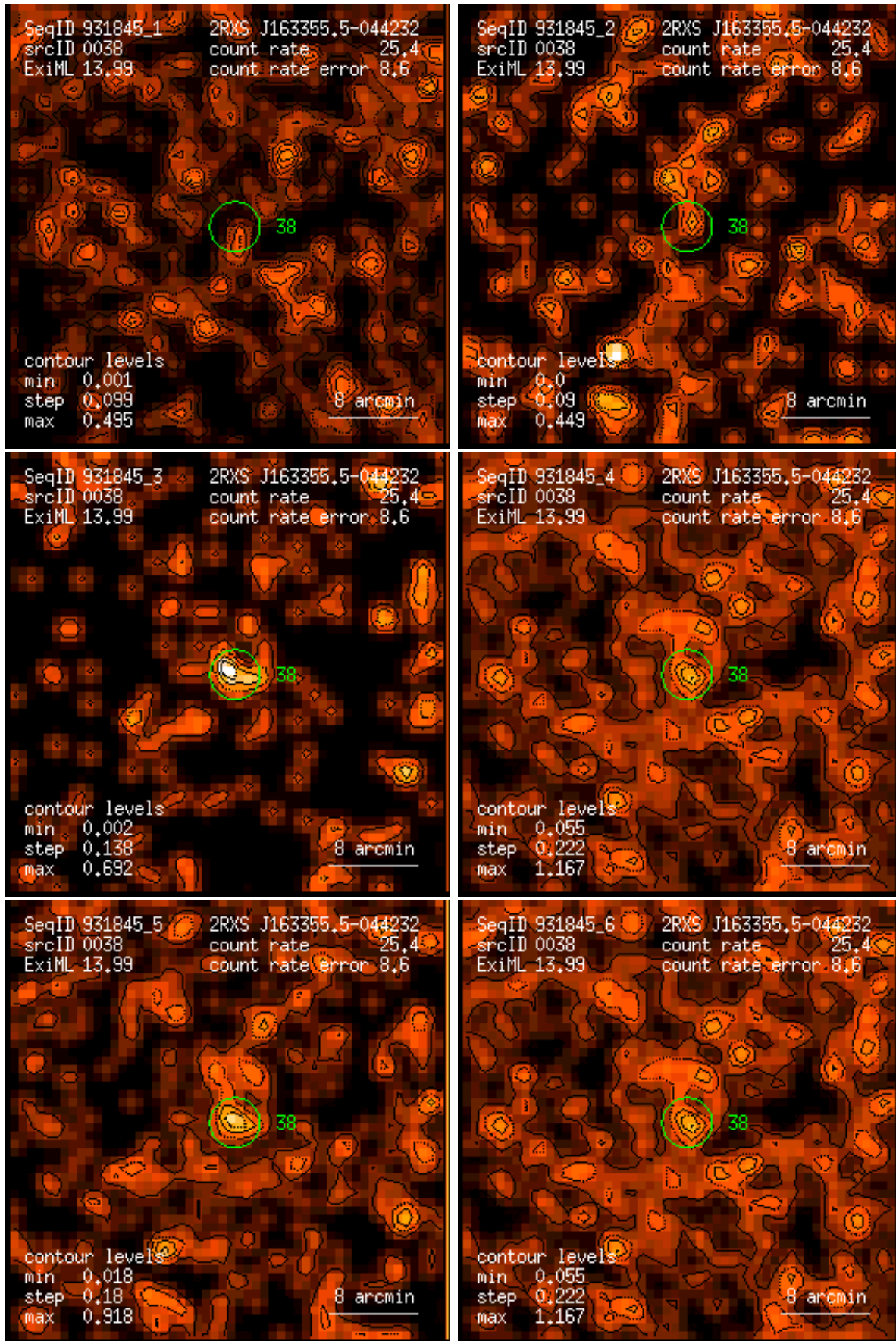
Figure 38: RASS 931845: detection 0038: band rate images, Gaussian filter: (1) PSPC channels 11 – 41, (2) 52 – 90, (3) 91 – 201, (4) 11 – 235, (5) 52 – 201, (6) 11 – 201. Broad band rates in counts/ks. Band rate contour levels in counts/ks/arcmin 2 .
