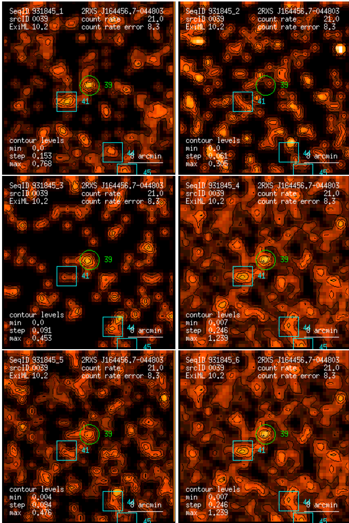
Figure 39: RASS 931845: detection 0039: band rate images, Gaussian filter: (1) PSPC channels 11 – 41, (2) 52 – 90, (3) 91 – 201, (4) 11 – 235, (5) 52 – 201, (6) 11 – 201. Broad band rates in counts/ks. Band rate contour levels in counts/ks/arcmin 2 .
