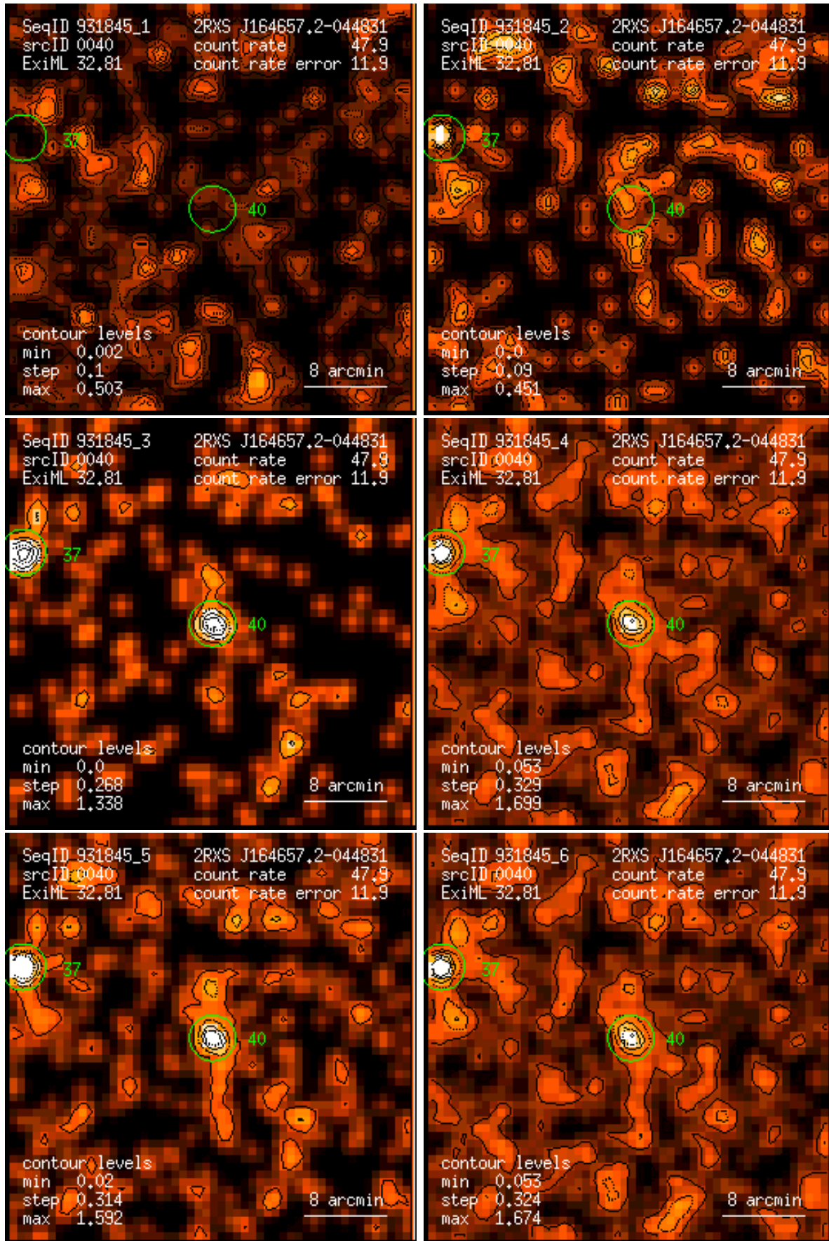
Figure 40: RASS 931845: detection 0040: band rate images, Gaussian filter: (1) PSPC channels 11 – 41, (2) 52 – 90, (3) 91 – 201, (4) 11 – 235, (5) 52 – 201, (6) 11 – 201. Broad band rates in counts/ks. Band rate contour levels in counts/ks/arcmin 2 .
