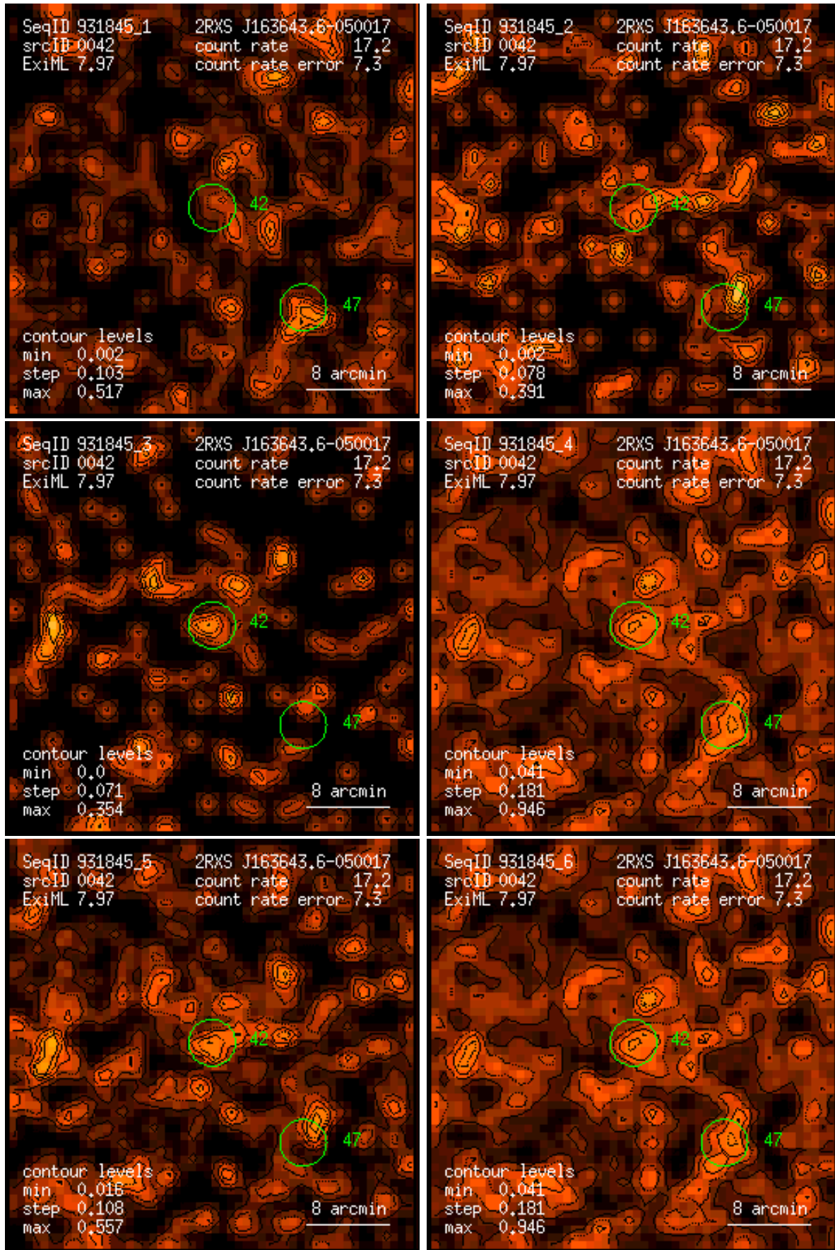
Figure 42: RASS 931845: detection 0042: band rate images, Gaussian filter: (1) PSPC channels 11 – 41, (2) 52 – 90, (3) 91 – 201, (4) 11 – 235, (5) 52 – 201, (6) 11 – 201. Broad band rates in counts/ks. Band rate contour levels in counts/ks/arcmin 2 .
