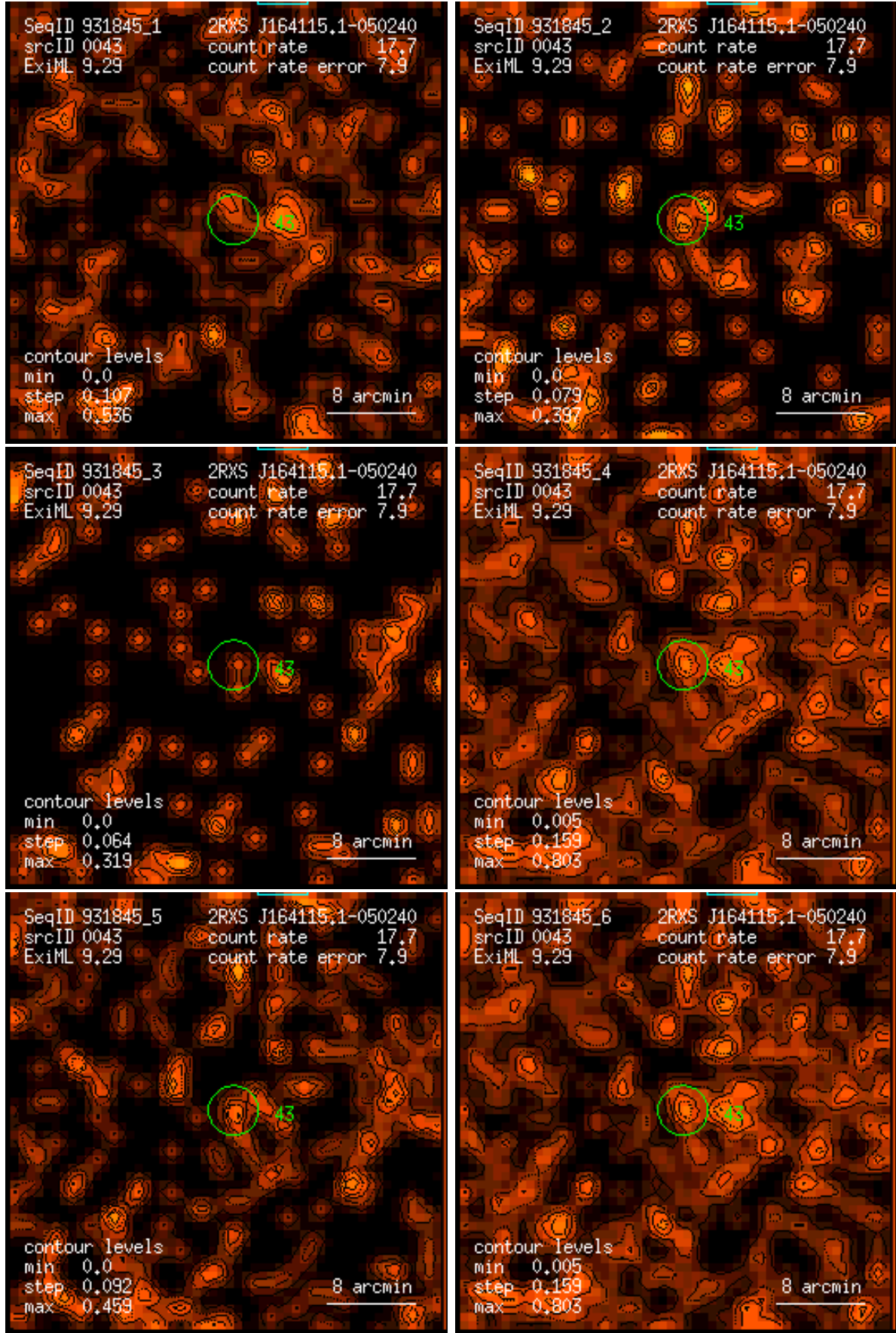
Figure 43: RASS 931845: detection 0043: band rate images, Gaussian filter: (1) PSPC channels 11 – 41, (2) 52 – 90, (3) 91 – 201, (4) 11 – 235, (5) 52 – 201, (6) 11 – 201. Broad band rates in counts/ks. Band rate contour levels in counts/ks/arcmin 2 .
