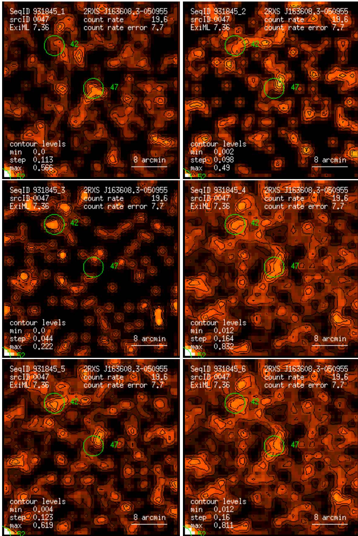
Figure 47: RASS 931845: detection 0047: band rate images, Gaussian filter: (1) PSPC channels 11 – 41, (2) 52 – 90, (3) 91 – 201, (4) 11 – 235, (5) 52 – 201, (6) 11 – 201. Broad band rates in counts/ks. Band rate contour levels in counts/ks/arcmin 2 .
