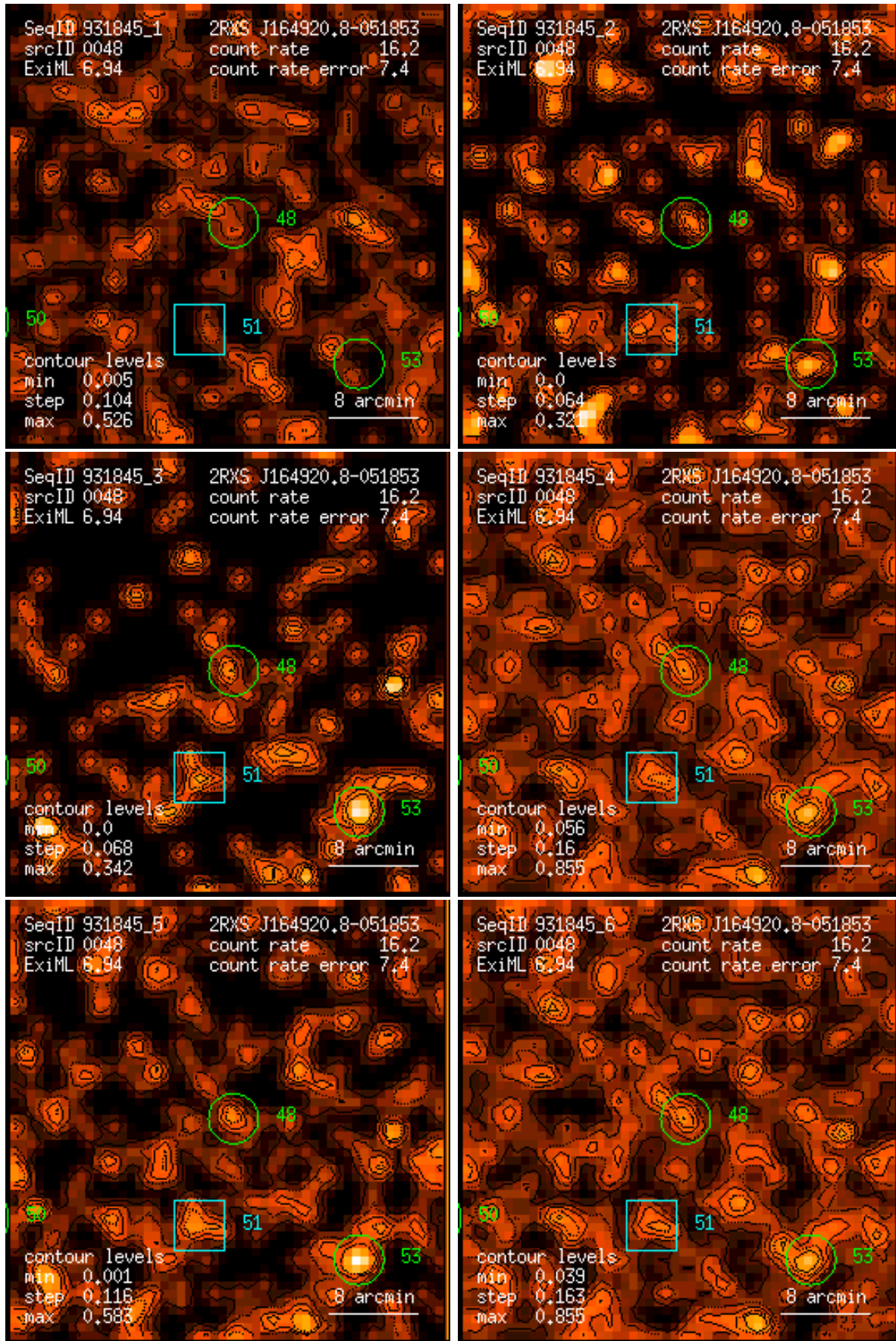
Figure 48: RASS 931845: detection 0048: band rate images, Gaussian filter: (1) PSPC channels 11 – 41, (2) 52 – 90, (3) 91 – 201, (4) 11 – 235, (5) 52 – 201, (6) 11 – 201. Broad band rates in counts/ks. Band rate contour levels in counts/ks/arcmin 2 .
