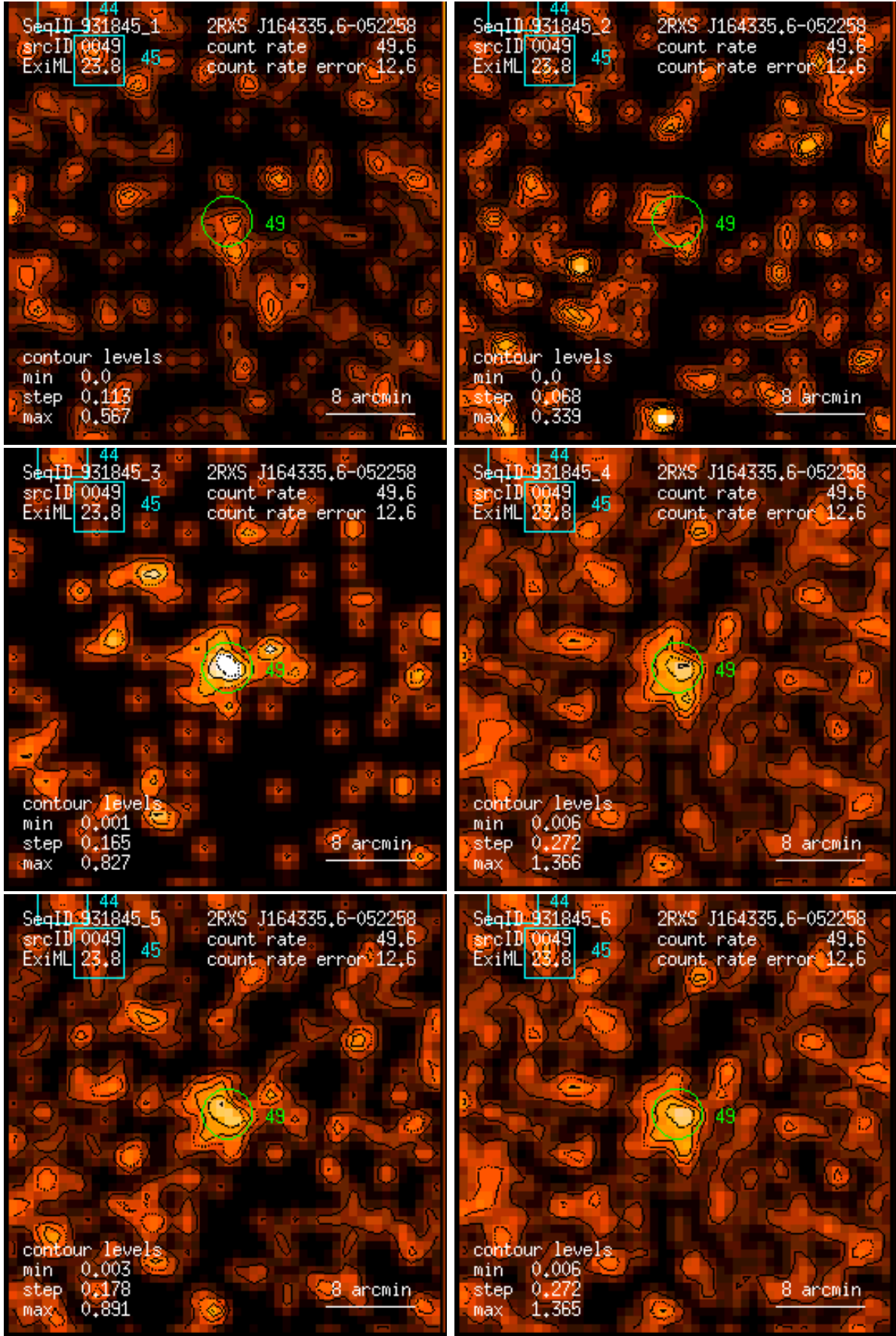
Figure 49: RASS 931845: detection 0049: band rate images, Gaussian filter: (1) PSPC channels 11 – 41, (2) 52 – 90, (3) 91 – 201, (4) 11 – 235, (5) 52 – 201, (6) 11 – 201. Broad band rates in counts/ks. Band rate contour levels in counts/ks/arcmin 2 .
