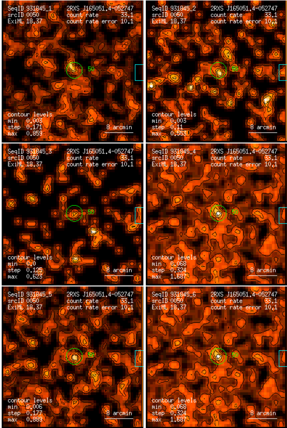
Figure 50: RASS 931845: detection 0050: band rate images, Gaussian filter: (1) PSPC channels 11 – 41, (2) 52 – 90, (3) 91 – 201, (4) 11 – 235, (5) 52 – 201, (6) 11 – 201. Broad band rates in counts/ks. Band rate contour levels in counts/ks/arcmin 2 .
