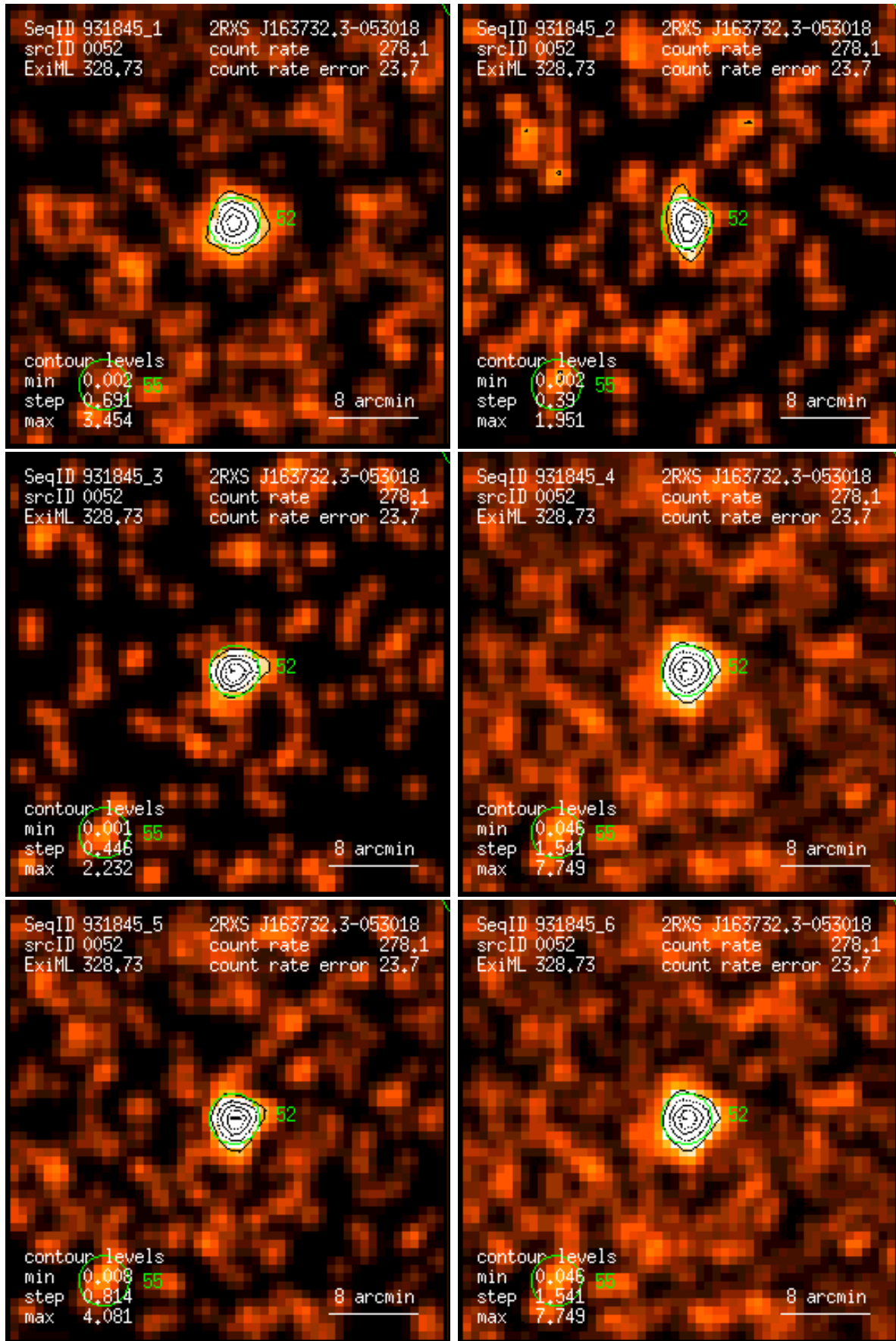
Figure 52: RASS 931845: detection 0052: band rate images, Gaussian filter: (1) PSPC channels 11 – 41, (2) 52 – 90, (3) 91 – 201, (4) 11 – 235, (5) 52 – 201, (6) 11 – 201. Broad band rates in counts/ks. Band rate contour levels in counts/ks/arcmin 2 .
