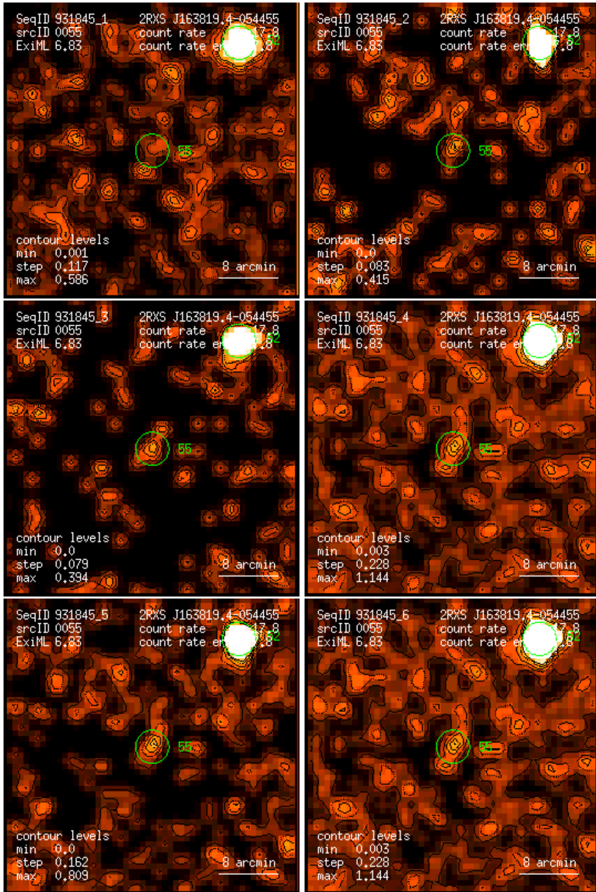
Figure 55: RASS 931845: detection 0055: band rate images, Gaussian filter: (1) PSPC channels 11 – 41, (2) 52 – 90, (3) 91 – 201, (4) 11 – 235, (5) 52 – 201, (6) 11 – 201. Broad band rates in counts/ks. Band rate contour levels in counts/ks/arcmin 2 .
