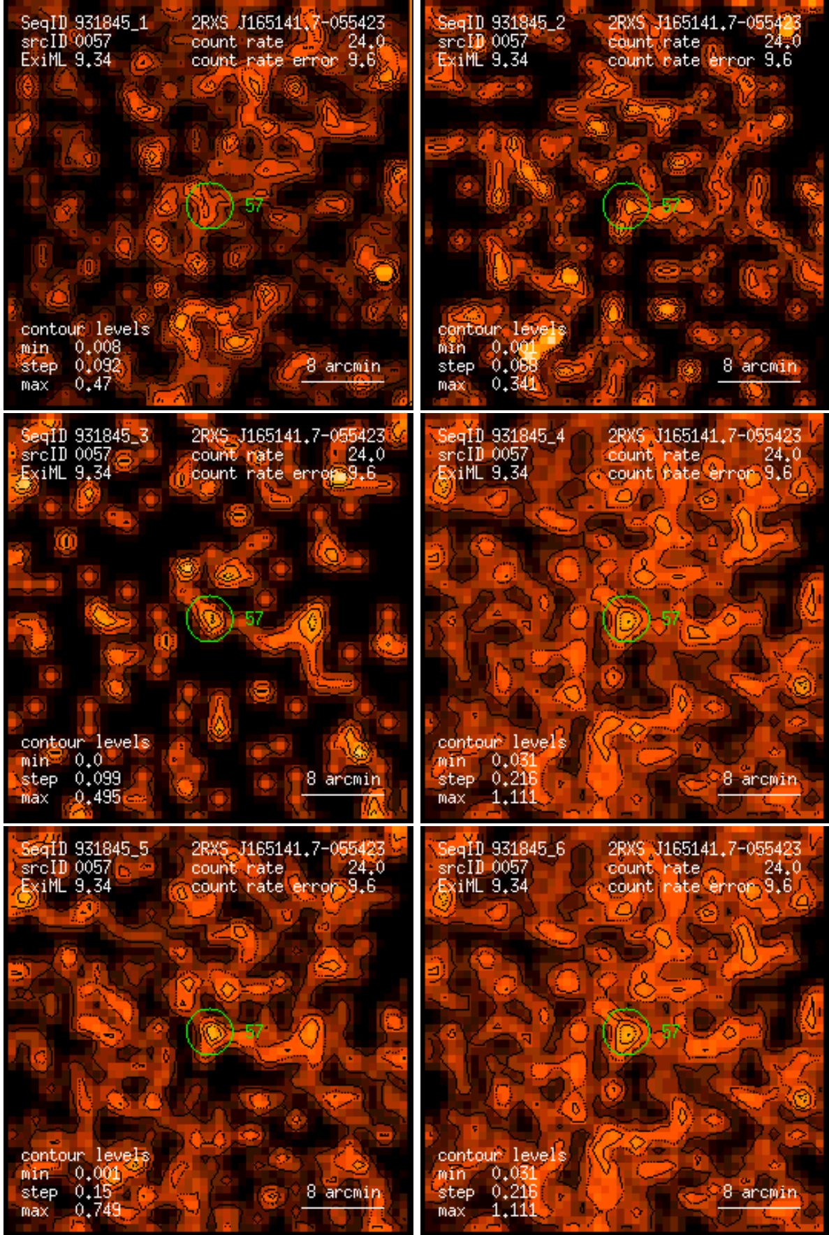
Figure 57: RASS 931845: detection 0057: band rate images, Gaussian filter: (1) PSPC channels 11 – 41, (2) 52 – 90, (3) 91 – 201, (4) 11 – 235, (5) 52 – 201, (6) 11 – 201. Broad band rates in counts/ks. Band rate contour levels in counts/ks/arcmin 2 .
