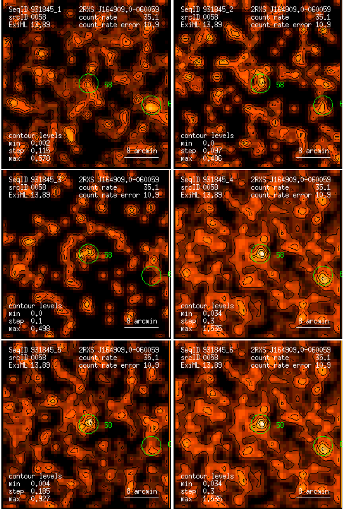
Figure 58: RASS 931845: detection 0058: band rate images, Gaussian filter: (1) PSPC channels 11 – 41, (2) 52 – 90, (3) 91 – 201, (4) 11 – 235, (5) 52 – 201, (6) 11 – 201. Broad band rates in counts/ks. Band rate contour levels in counts/ks/arcmin 2 .
