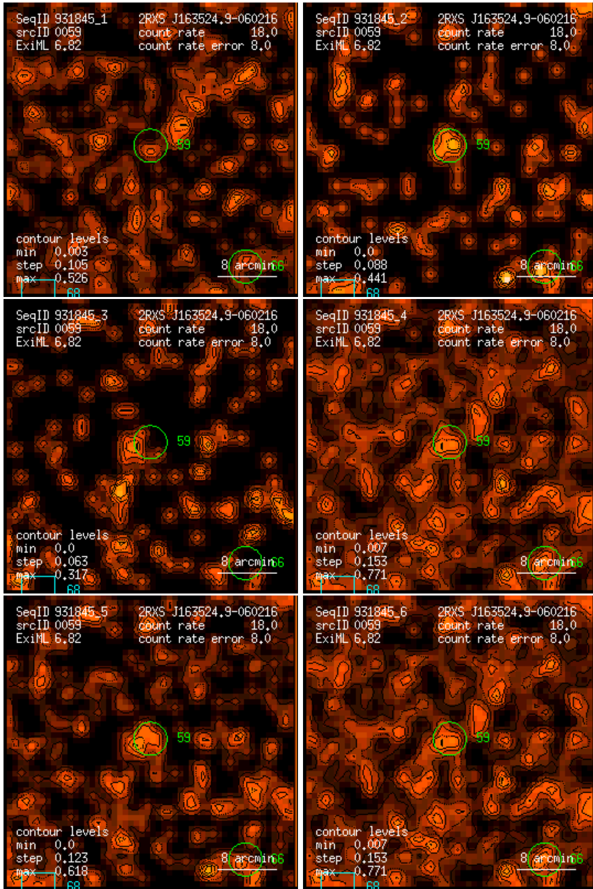
Figure 59: RASS 931845: detection 0059: band rate images, Gaussian filter: (1) PSPC channels 11 – 41, (2) 52 – 90, (3) 91 – 201, (4) 11 – 235, (5) 52 – 201, (6) 11 – 201. Broad band rates in counts/ks. Band rate contour levels in counts/ks/arcmin 2 .
